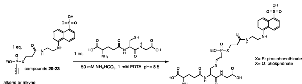
Scheme 8: Conjugation of glutathione to fluorescent alkene- and alkyne phosphonothiolates and phosphonates.
