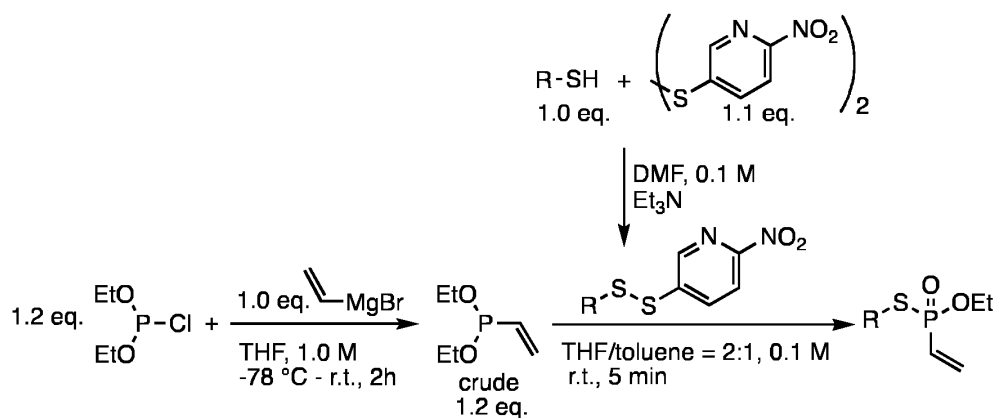
Scheme 3: Synthesis of O-ethyl alkene-phosphonothiolates from the reaction of diethyl alkenephosphonite with electrophilic disulfides.
