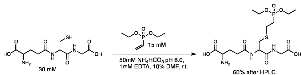
Scheme 1: Synthesis of glutathione-phosphonate conjugate.
