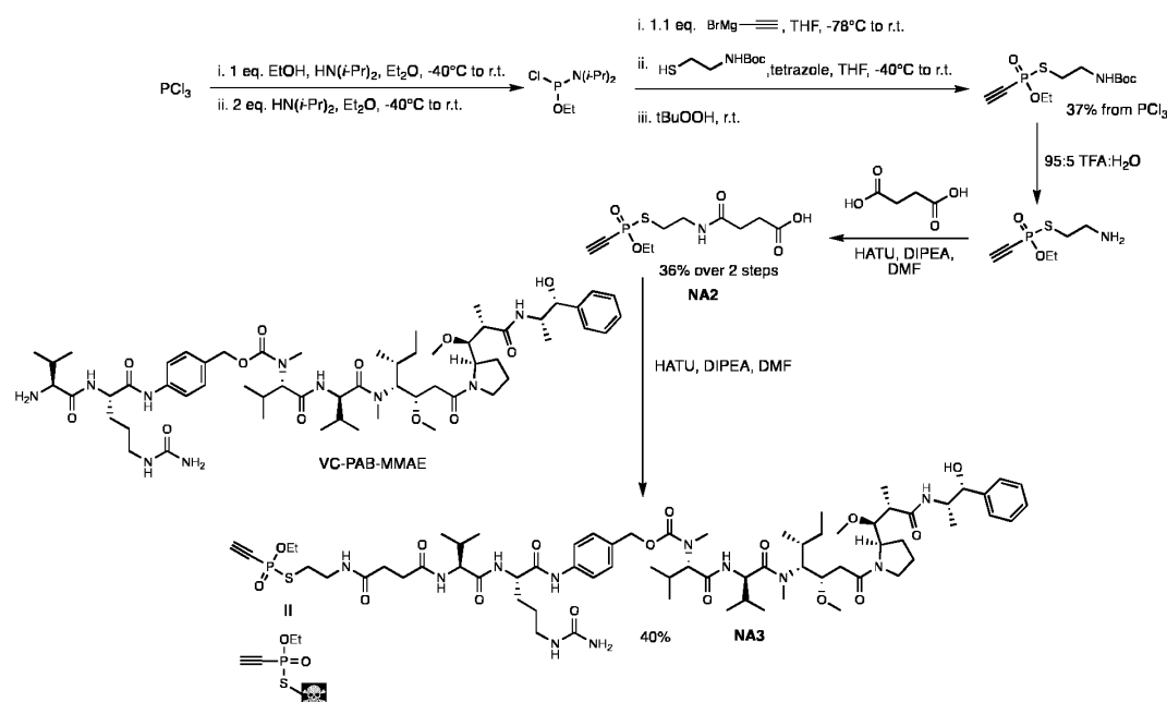
Scheme 12: Synthetic route for the construction of phosphonothiolate linked, cathepsin B cleavable monomethyl auristatin E conjugate NA3 . VC: Valine-citrullin dipeptide, PAB: p -aminobenzyl.
