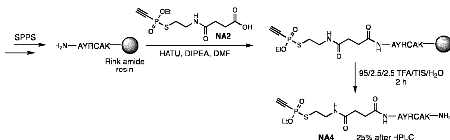
Scheme 13: Solid phase peptide synthesis using alkyne phosphonothiolate.
