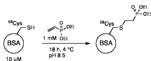
Scheme 10: Modification of BSA with diethyl alkenephosphonate.
