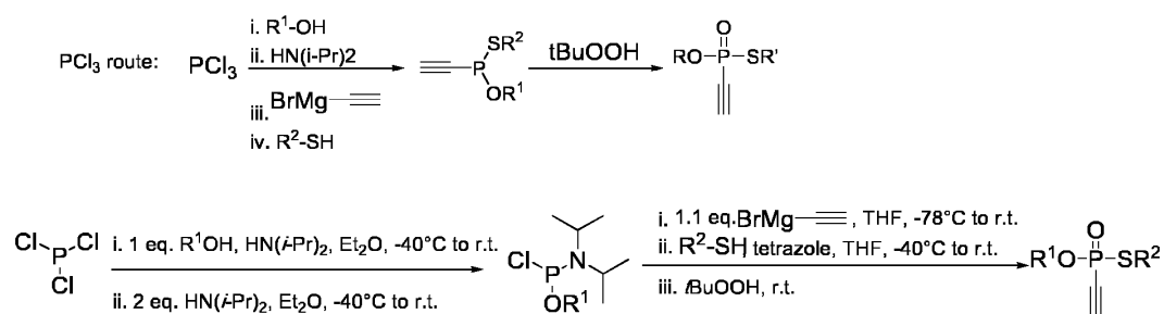
Scheme 5: Synthesis of alkyne-phosphonothiolates via the \text{PCl}_3 route.
