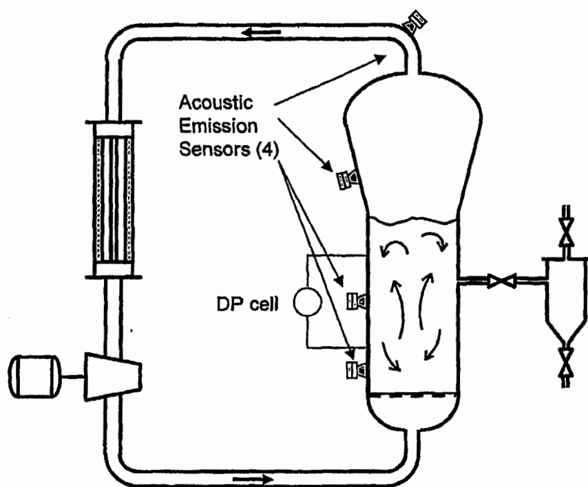
Figure 1 – Pilot Scale Fluidized Bed Reactor
