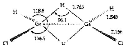
III. cis 1,2 C_{2v} structure
