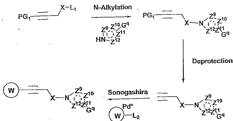
Scheme 23
