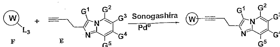
Scheme 17
