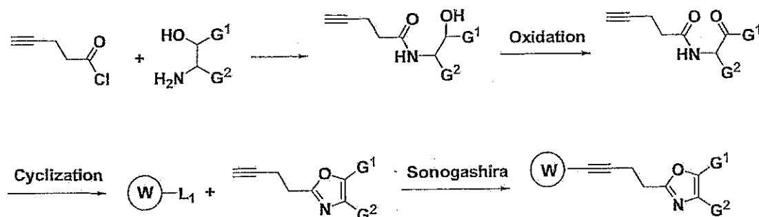
Scheme 36
