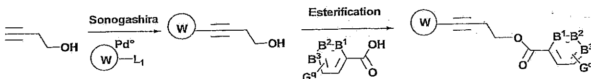
Scheme 24
