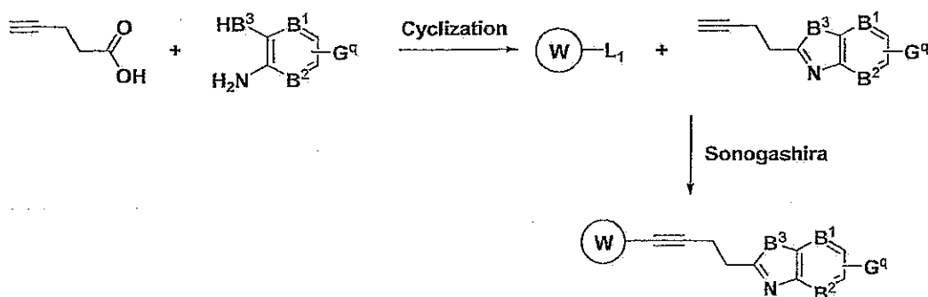
Scheme 32
