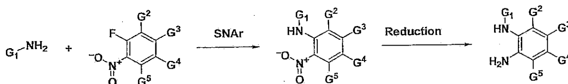
Scheme 18
