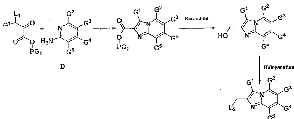
Scheme 11
