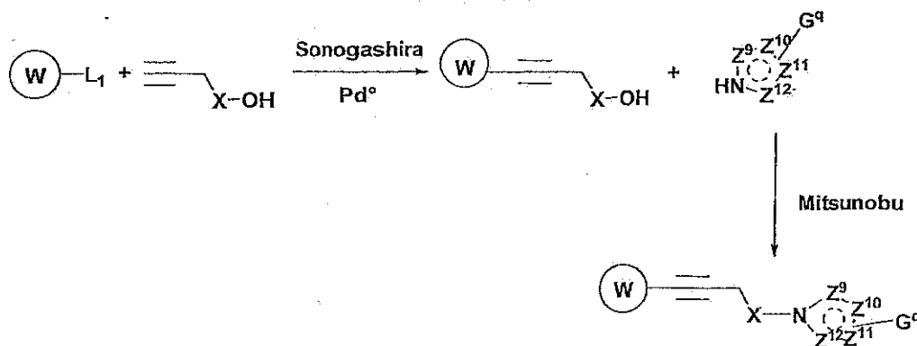
Scheme 21
