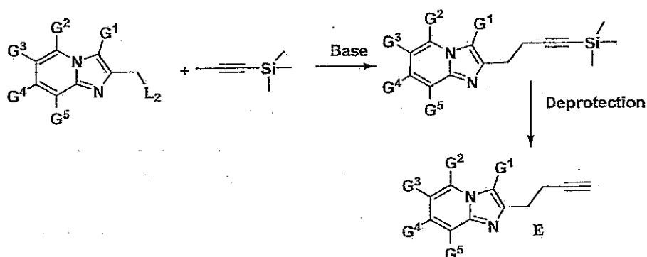
Scheme 13
