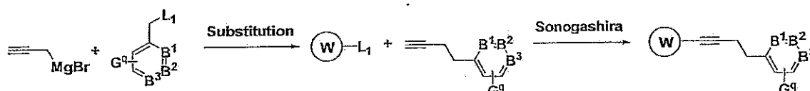
Scheme 37
