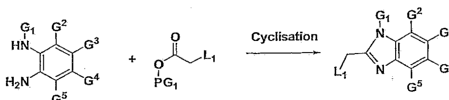
Scheme 19
