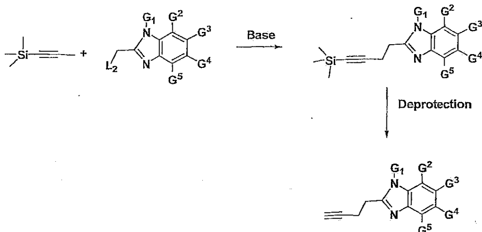
Scheme 20
