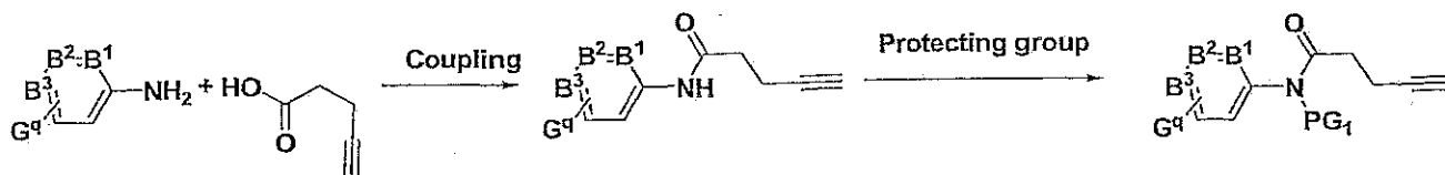
Scheme 26
