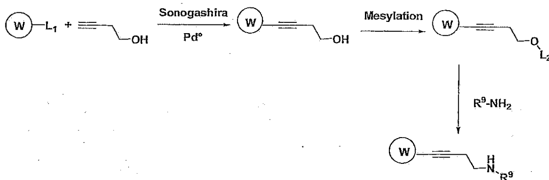
Scheme 28
