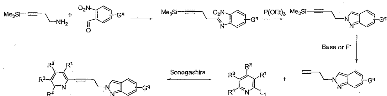
Scheme 34
