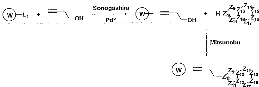
Scheme 30
