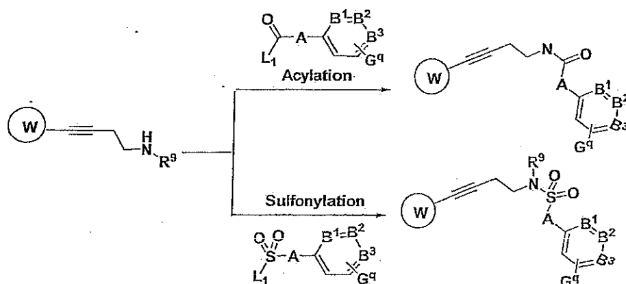
Scheme 29
