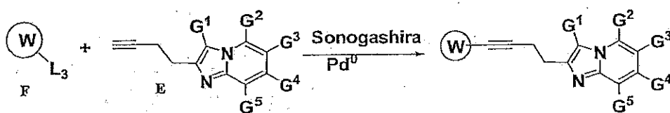
Scheme 14
