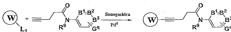
Scheme 7
