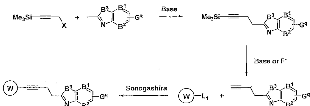
Scheme 33
