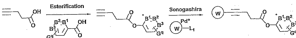
Scheme 25
