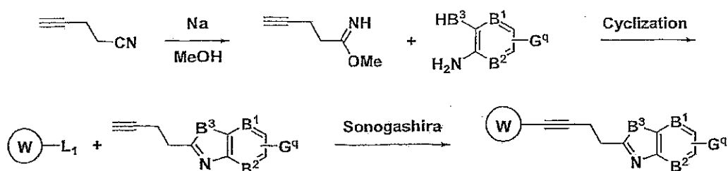
Scheme 31
