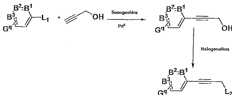
Scheme 8
