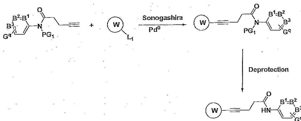
Scheme 27
