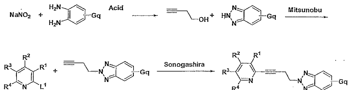
Scheme 35
