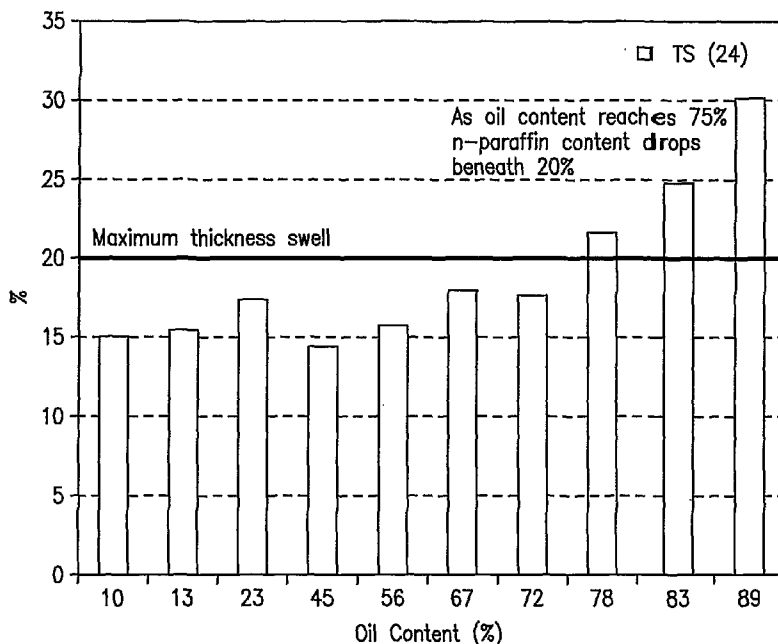
Effect Of Oil Content on Thickness Swell (24 hr)
