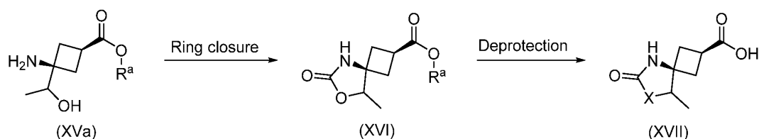
SCHEME 5
