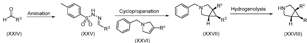
SCHEME 9
