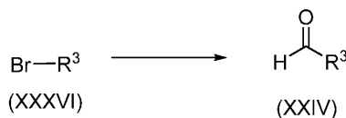
SCHEME 13
