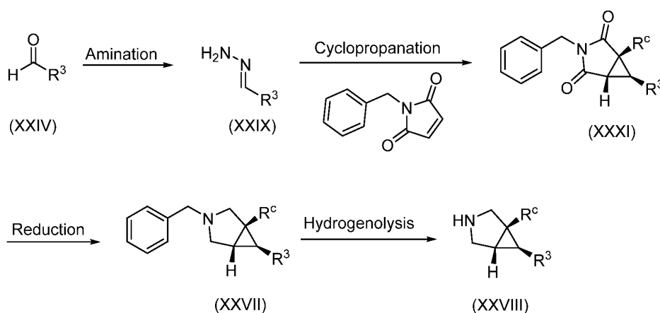
SCHEME 10
