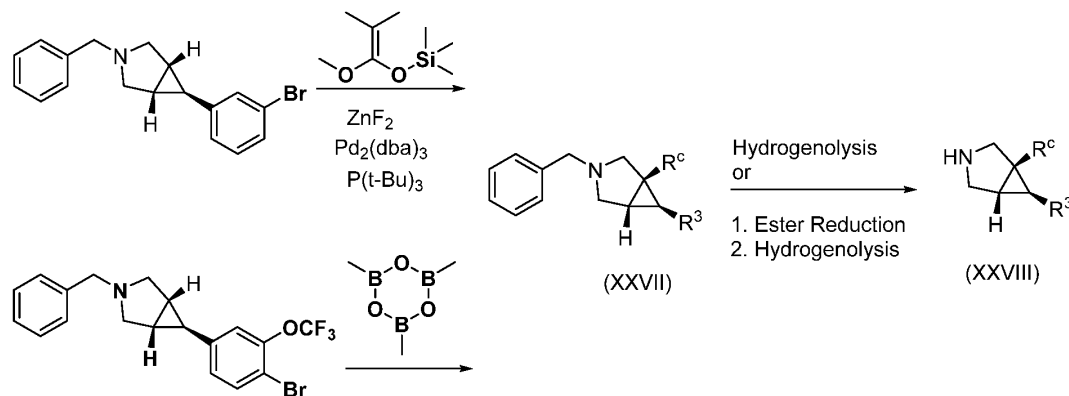
SCHEME 15
