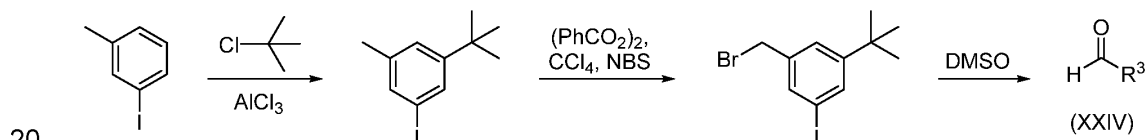
SCHEME 14
