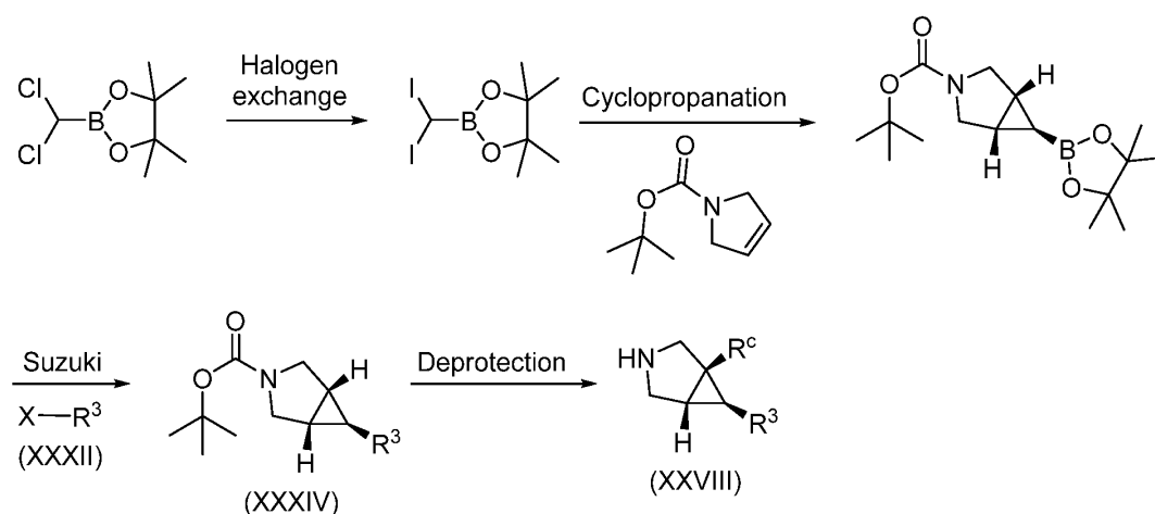
SCHEME 11
