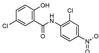
Niclosamide: 5-chloro- N -(2-chloro-4-nitrophenyl)-2-hydroxybenzamide
