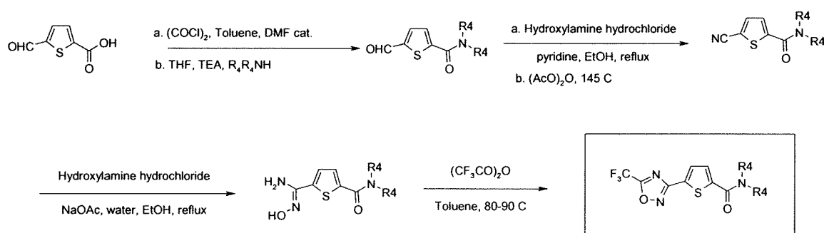
Scheme 7
