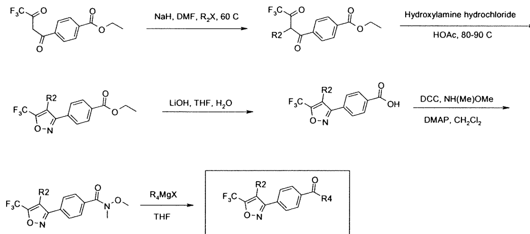
Scheme 6
