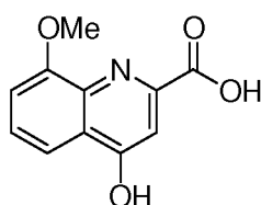
8-methoxykynurenic acid
