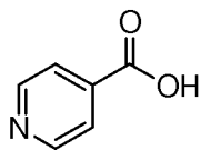
isonicotinic acid
