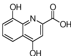
xanthurenic acid
