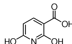
2,6-dihydroxynicotinic acid
