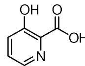
3-hydroxypicolinic acid
