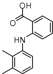
Mefenamic acid
