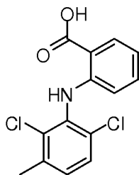
Meclofenamic acid
