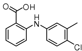
Tolfenamic acid
