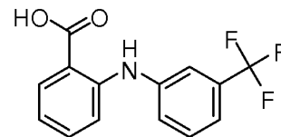
Flufenamic acid
