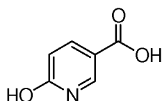
6-hydroxynicotinic acid
