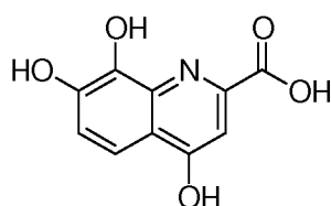
7,8-dihydroxykynurenic acid
