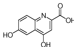
6-hydroxy-kynurenic acid
