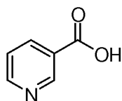
nicotinic acid
