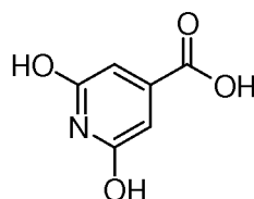
citrazinic acid
