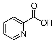
picolinic acid
