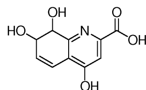
7,8-dihydro-7,8-dihydroxykynurenic acid
