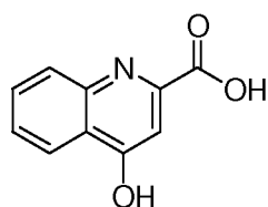
kynurenic acid
