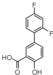
Diflusal
