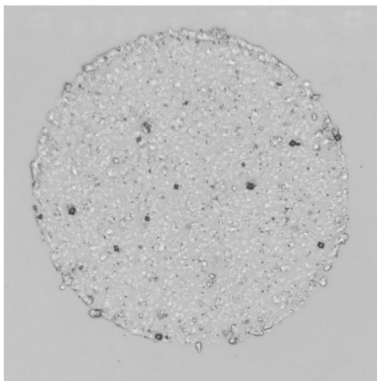
Synthetic Example 12
