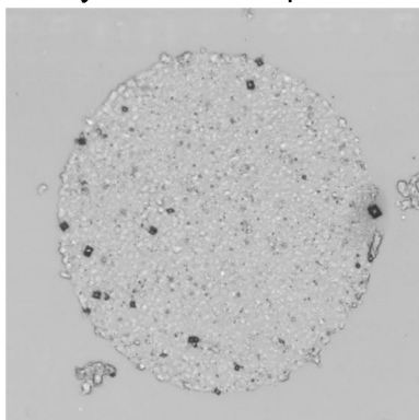
Synthetic Example 11
