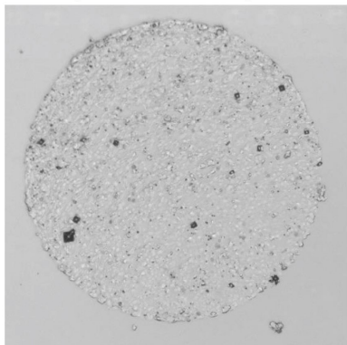
Synthetic Example 11
