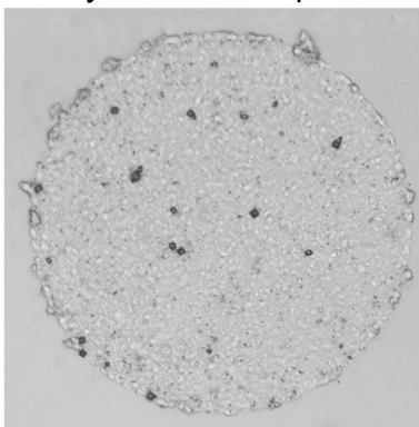
Synthetic Example 12
