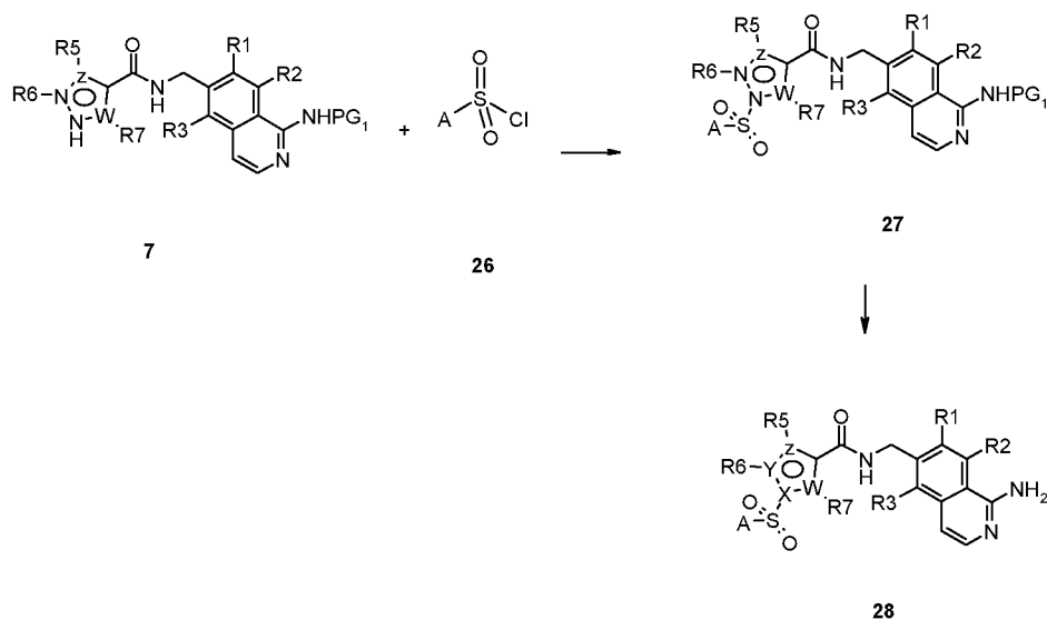
Scheme 7
