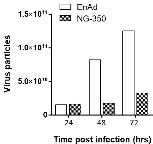
Figure 2 Total Virus Production (A) & Virus in the Supernatant (B)
