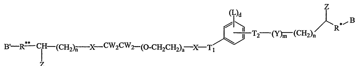
Formula XXI:
