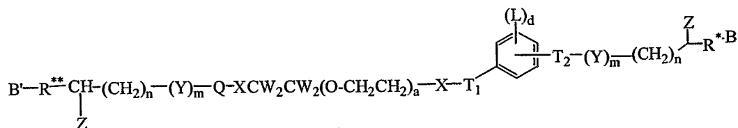
Formula XXI:
