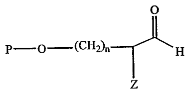
Formula XI:
