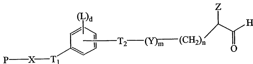
Formula VI
