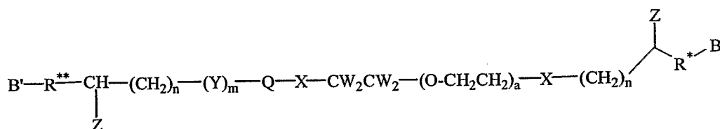
Formula XXV:
