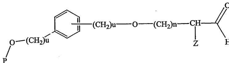
Formula IX:
