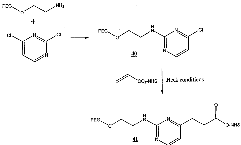
Scheme XV
