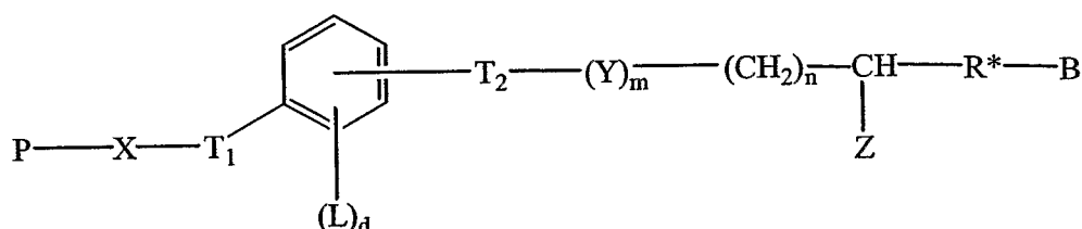
Formula XV:
