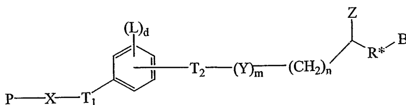
Formula XVI
