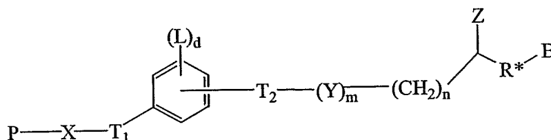
Formula XVI:
