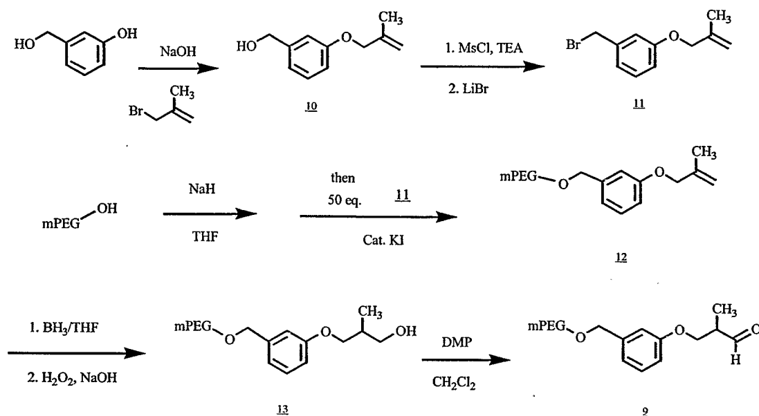
Scheme V:
