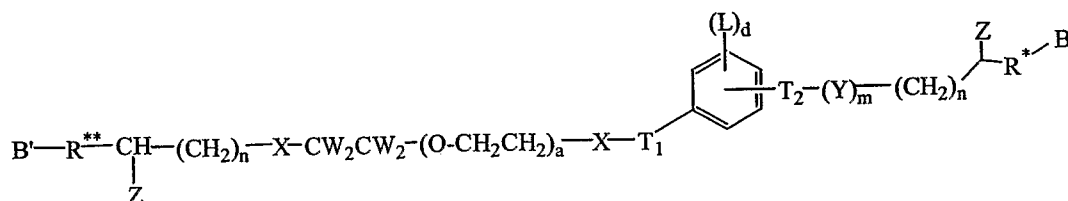
Formula XXI:
