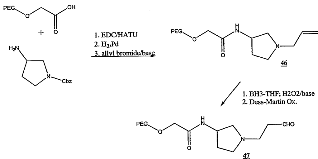
Scheme XVII
