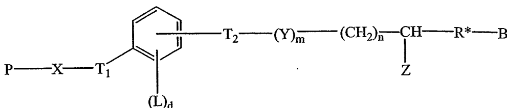
Formula XV:
