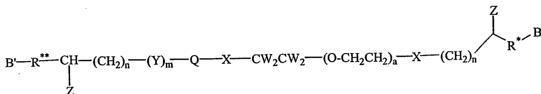
Formula XXIV:
