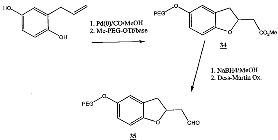
Scheme XII
