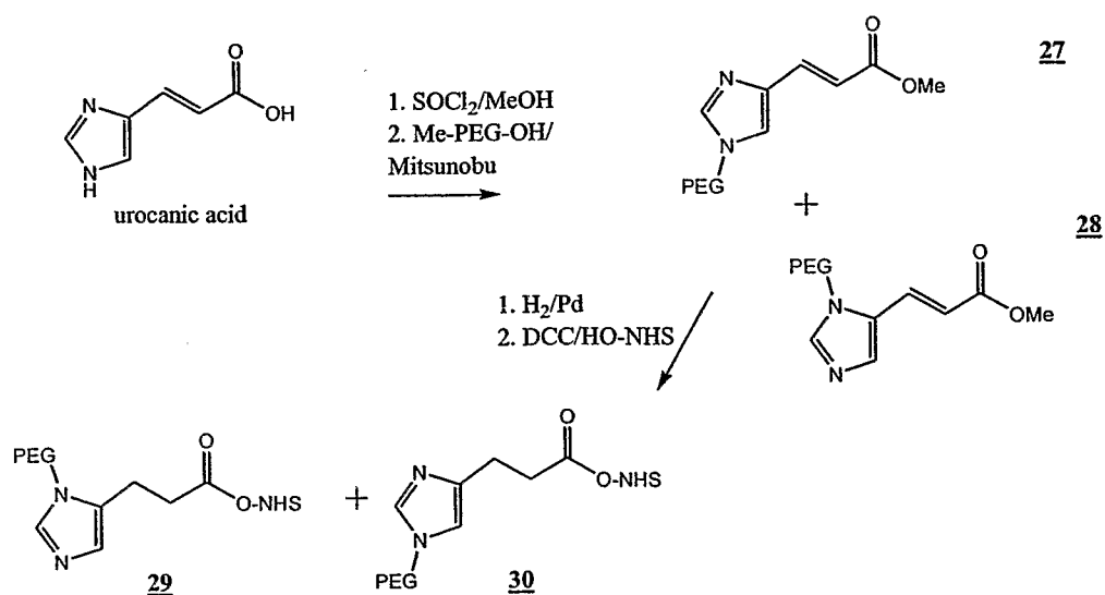
Scheme X
