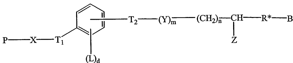
Formula XV
