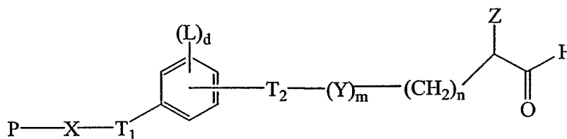
Formula VI
