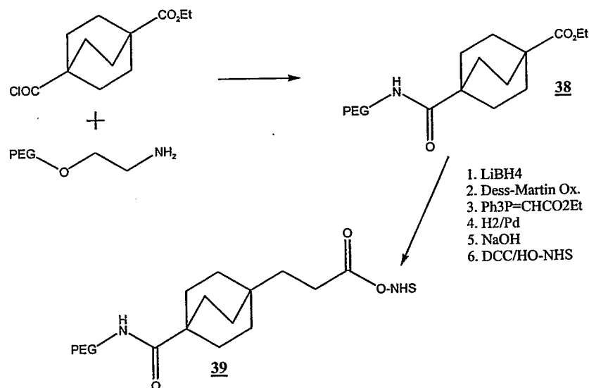
Scheme XIV
