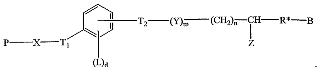
Formula XV
