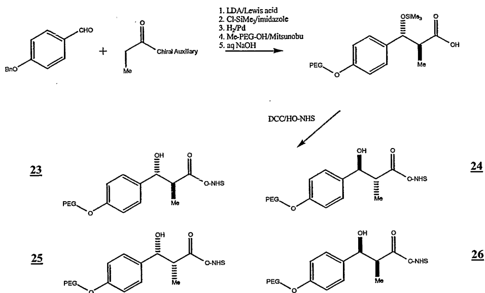
Scheme IX
