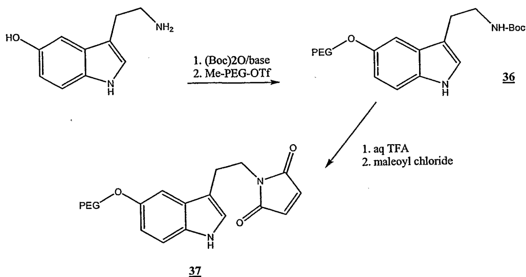
Scheme XIII
