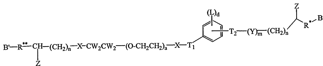
Formula XXI:
