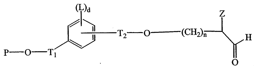
Compound J
