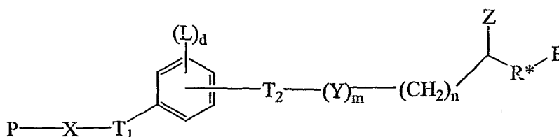
Formula XVI
