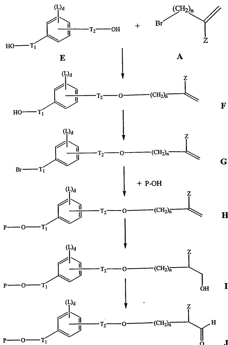
Scheme III
