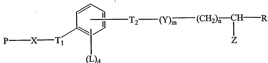
Formula V
