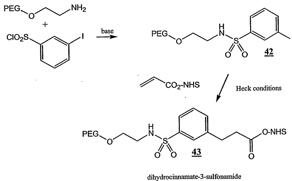
Scheme XVI
