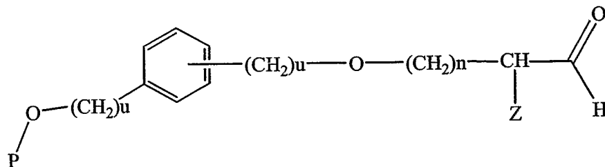
Formula IX:
