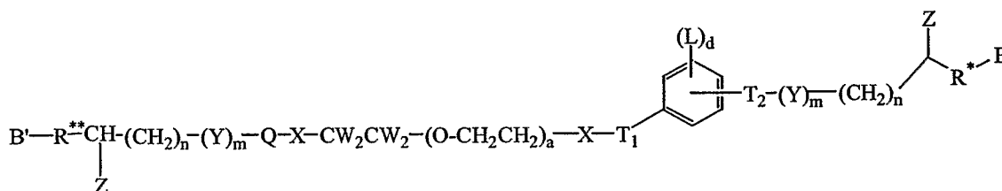
Formula XX:
