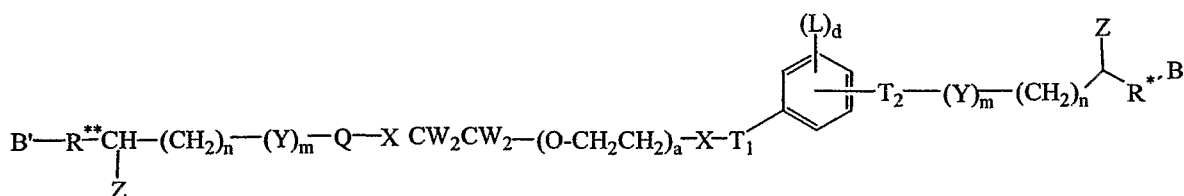
Formula XX:
