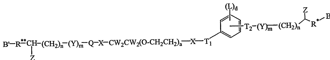
Formula XXI:
