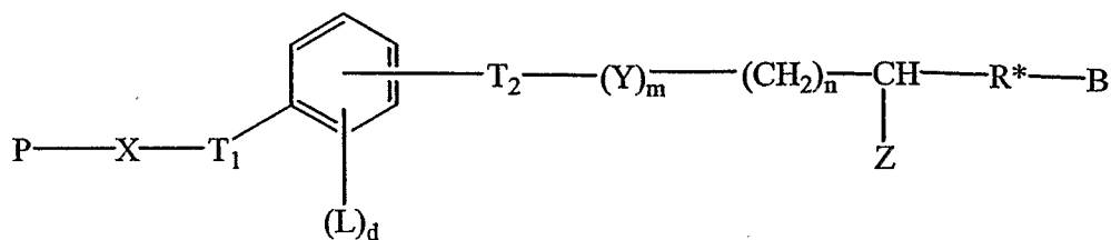
Formula XV:
