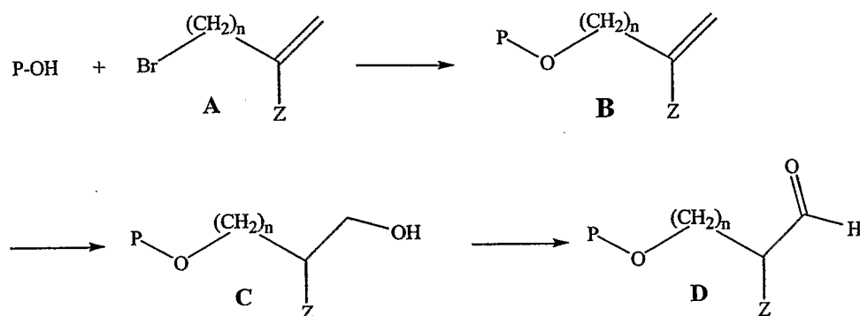
Scheme I
