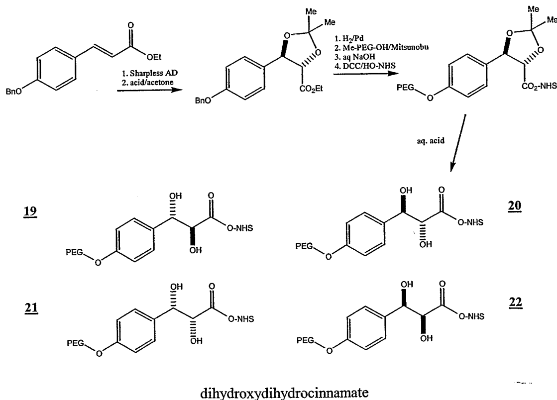
Scheme VIII
