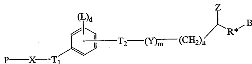
Formula XVI
