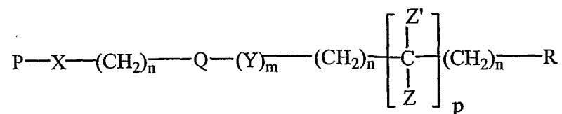
Formula I
