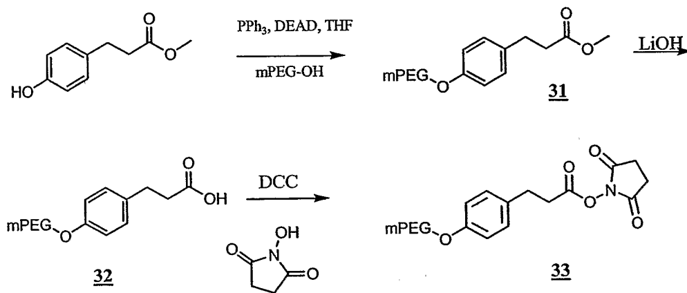
Scheme XI
