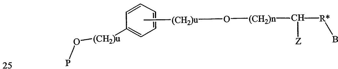
Formula XIX:
