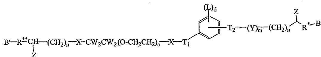
Formula XXI:
