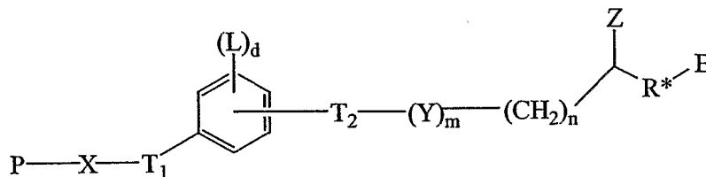
Formula XVI:
