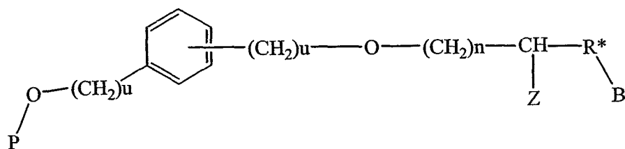
Formula XIX:
