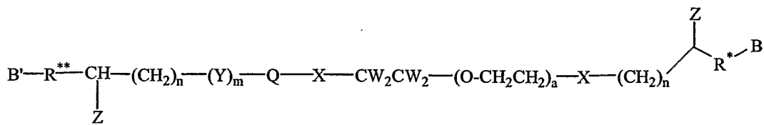
Formula XXIV:
