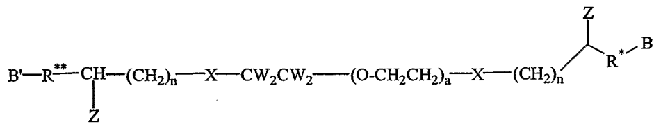
Formula XXV:
