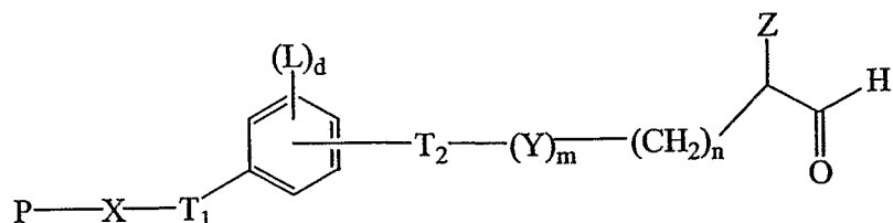
Formula VI
