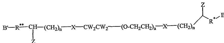
Formula XXV:
