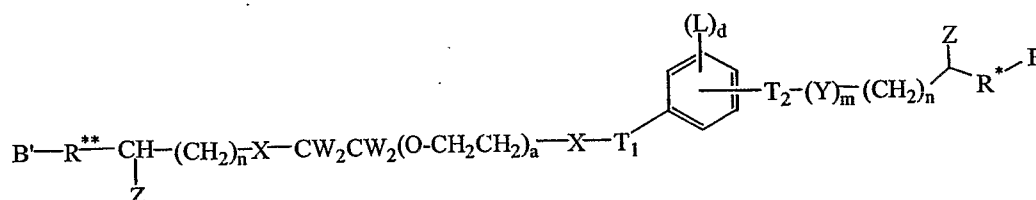
Formula XXI:
