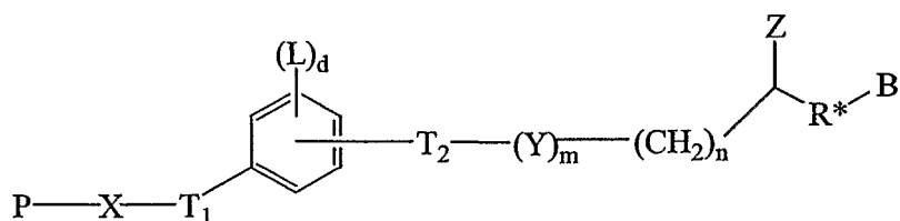
Formula XVI
