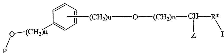
Formula XIX:
