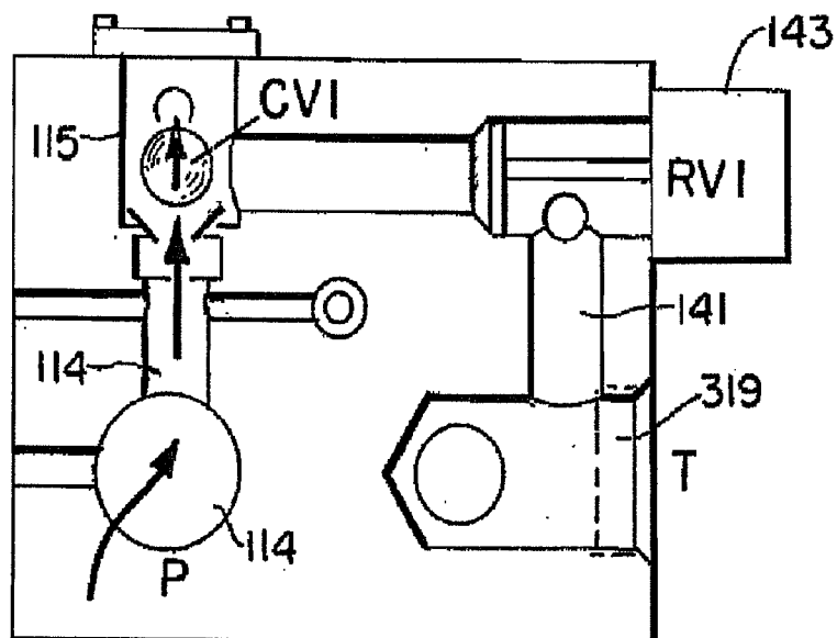
FIG. 42. UP STROKE
