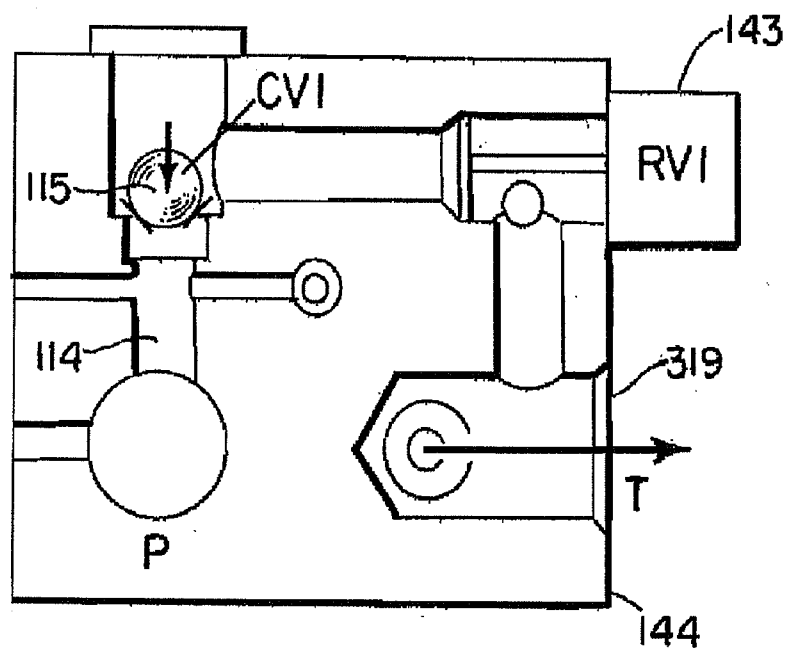
FIG. 38. DOWN STROKE
