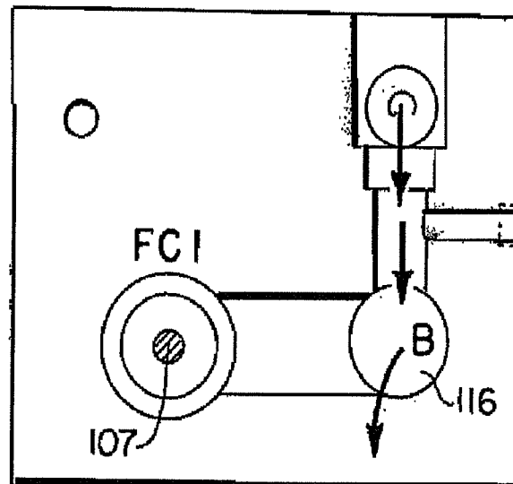
FIG. 41. UP STROKE
