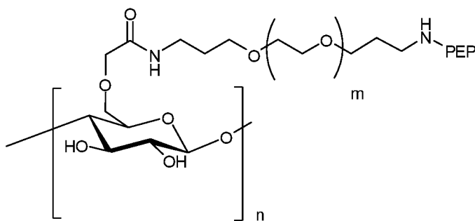
Formula IIc
