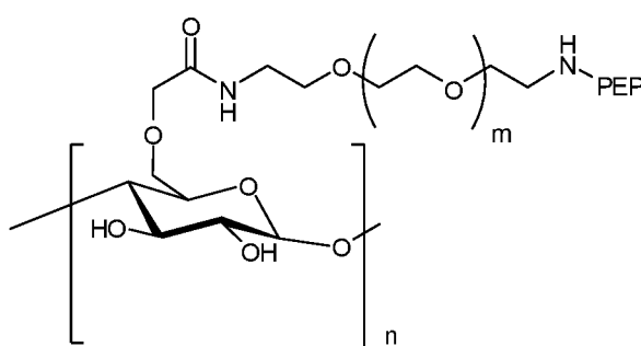
Formula IIb
