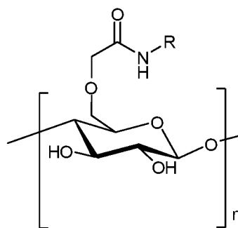
Formula Ib
