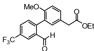
Formula IV
