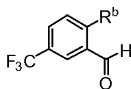
Formula VII
