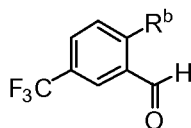
Formula VII
