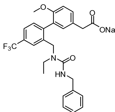
(Compound 2).
