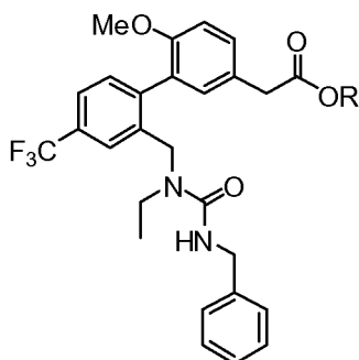
Formula VI;
