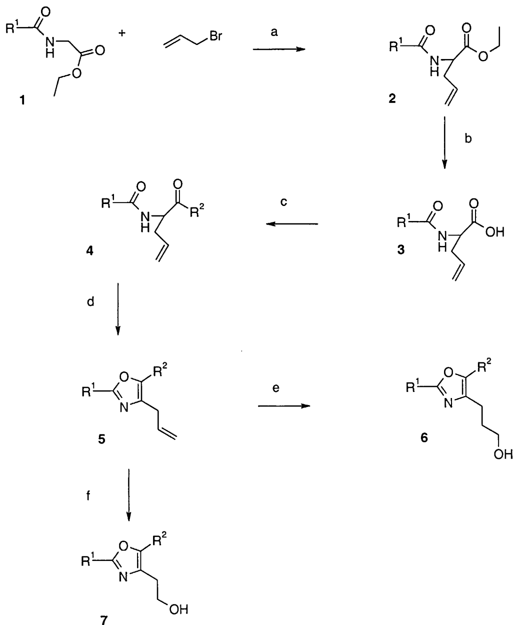
Scheme 13
