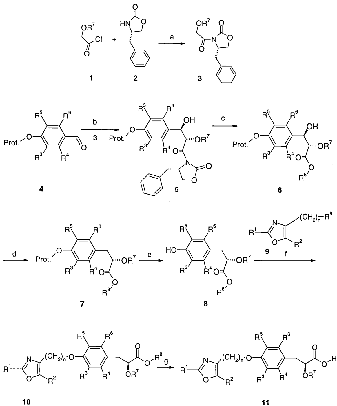
Scheme 1
