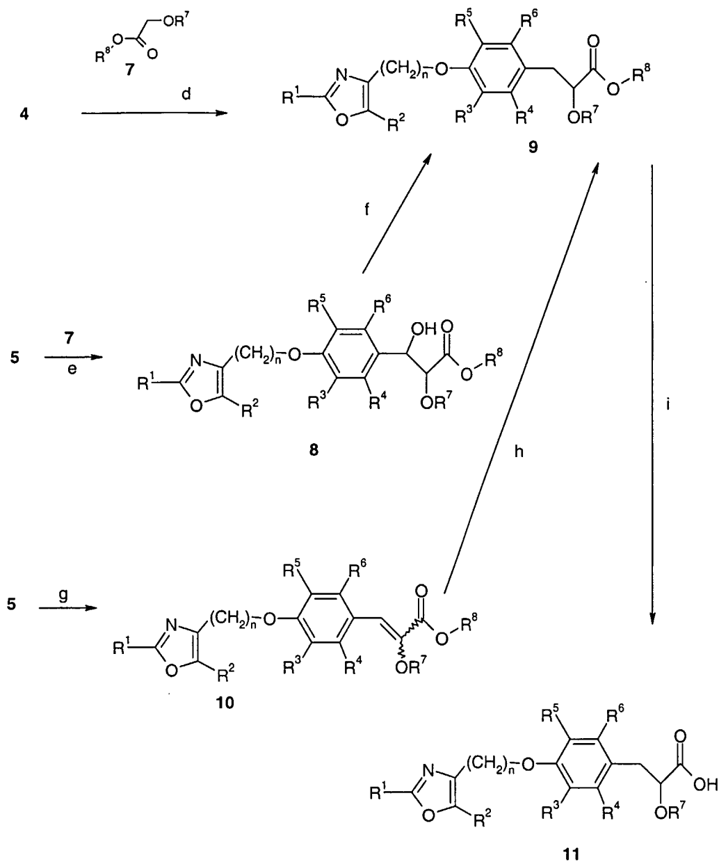
Scheme 4, Part II
