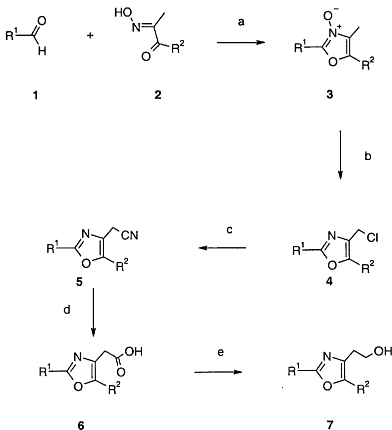
Scheme 12
