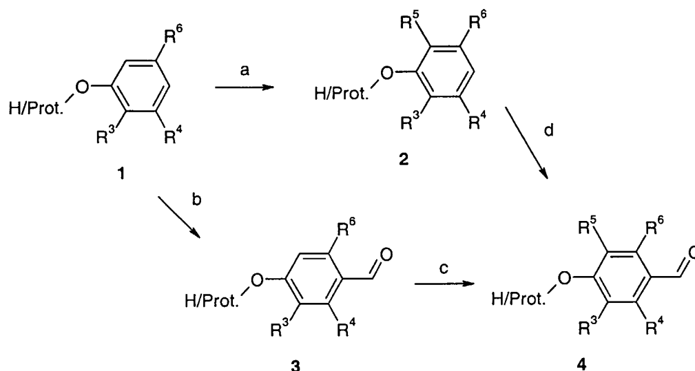
Scheme 11
