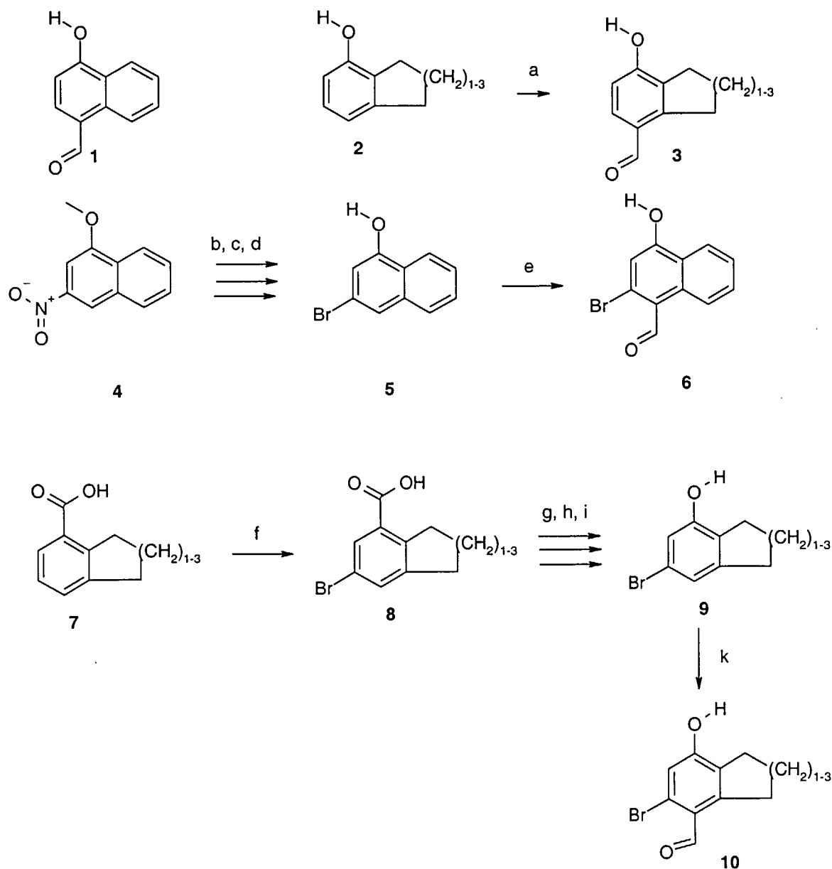
Scheme 8
