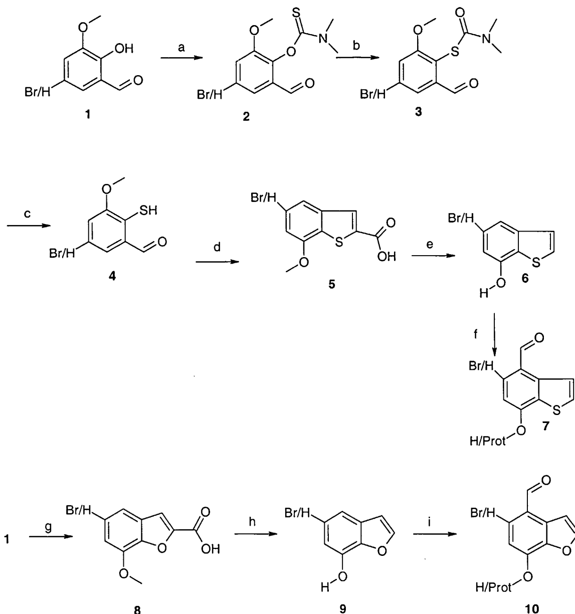
Scheme 7
