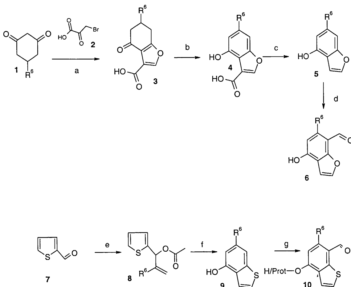
15 Scheme 6
