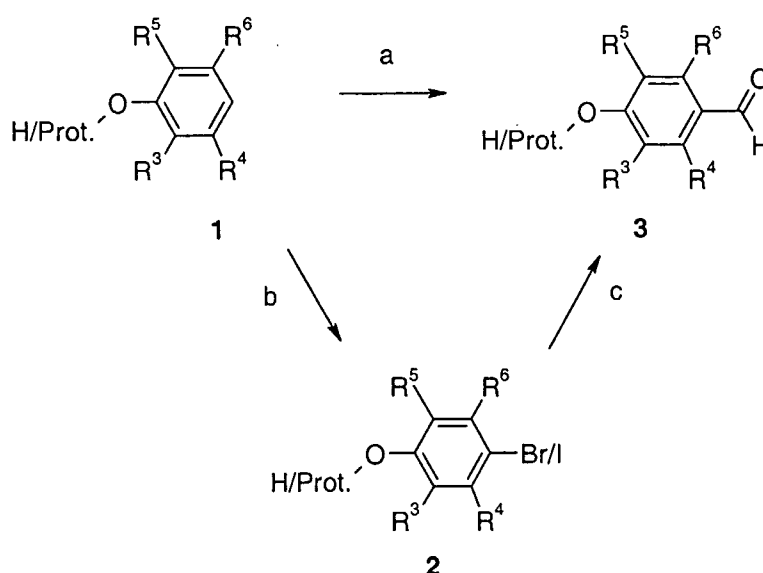
Scheme 5
