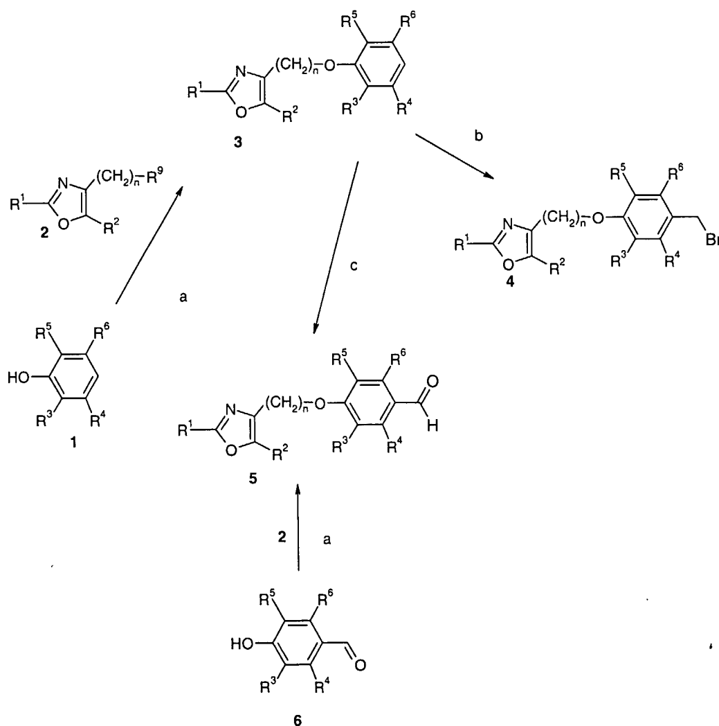
Scheme 4, Part I
