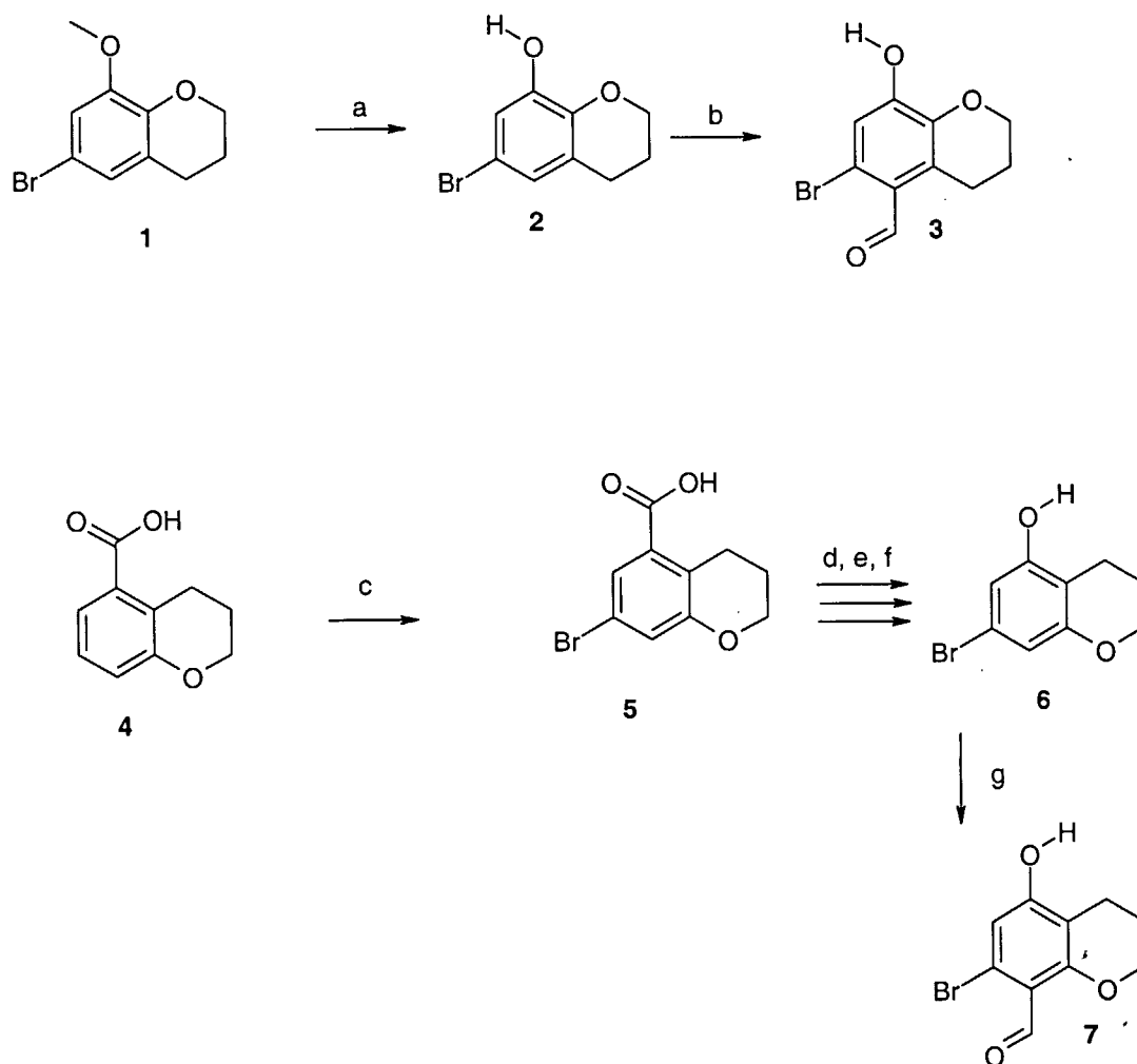
Scheme 9
