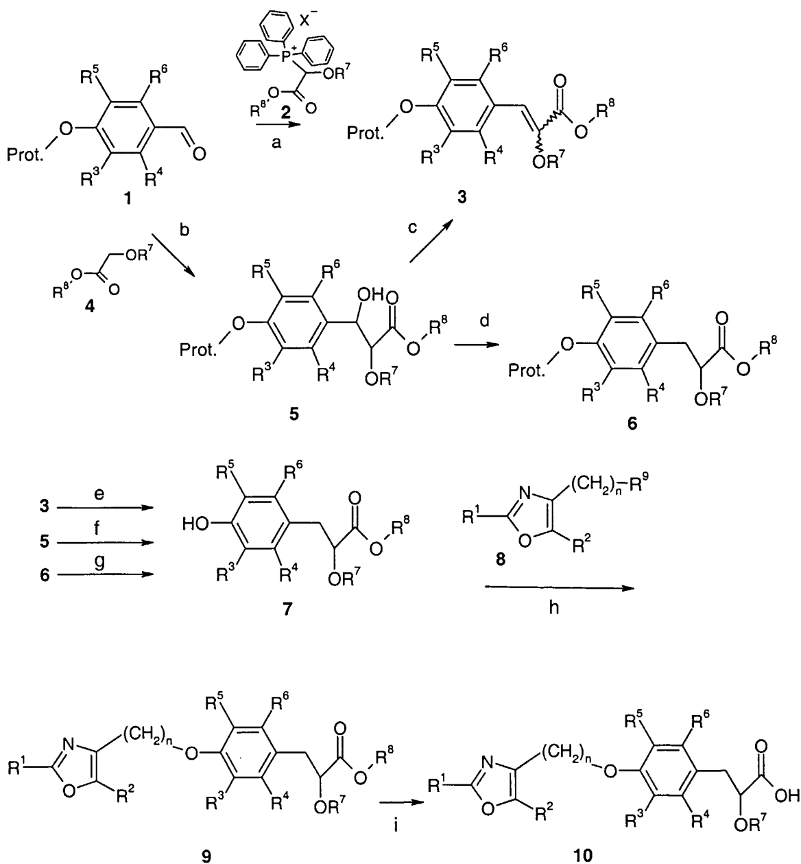
Scheme 2
