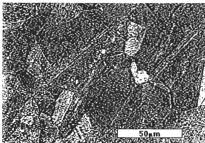
Figure 2a: Microstructure of conventionally manufactured NiFeNb alloy.
