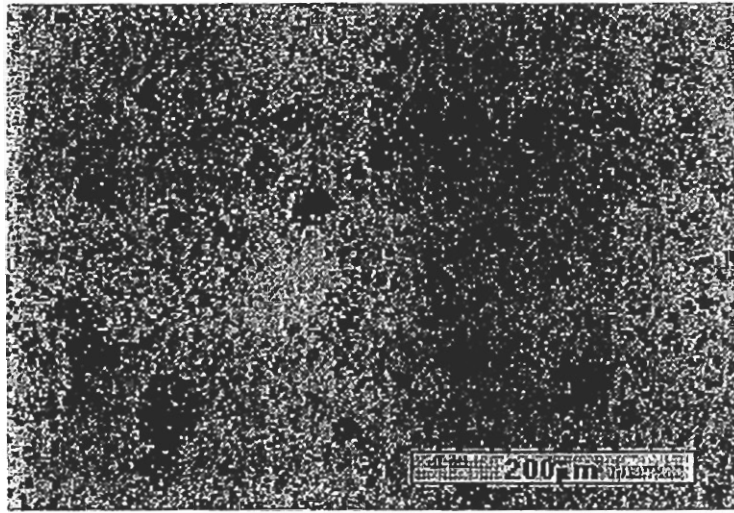
Figure 3a: PMP processed FeAlSi using elemental phases (Fe - white, Al - large gray and Si - small gray particles).
