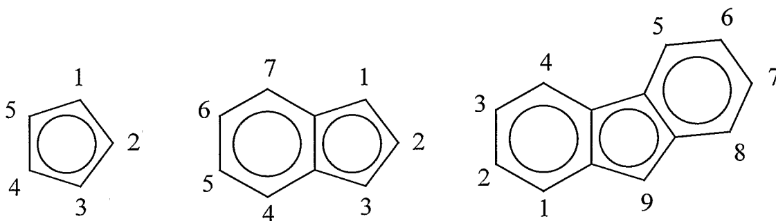
Cyclopentadienyl
