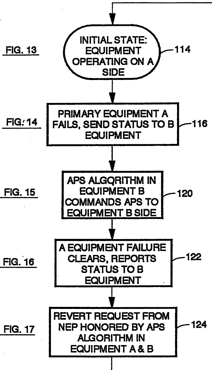
FIG. 12 PAYLOAD PATH EQUIPMENT FAILURE
