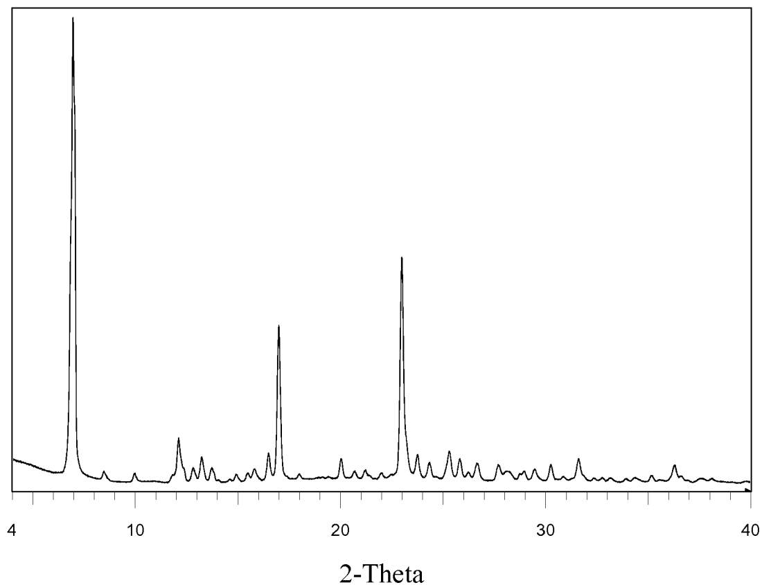
X-ray powder diffraction pattern of Example 1F, 2-chloro-4-[[ (1R,2R) -2-hydroxy-2-methyl-cyclopentyl]amino]-3-methyl-benzonitrile crystalline isopropanol solvate.
