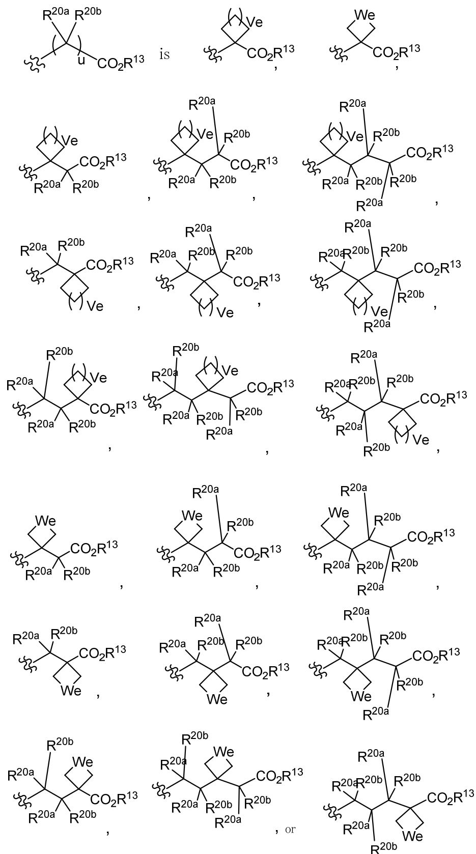
[Chemical Formula 28]
