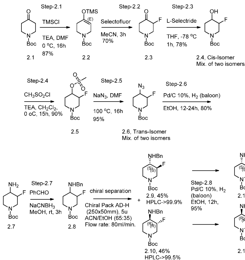
Scheme 5:
