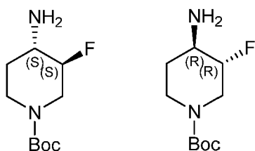
Scheme 5:
