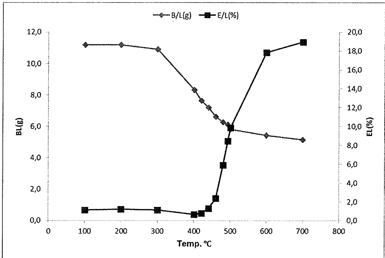
Fig.1 Annealing curve of wire sample 1
