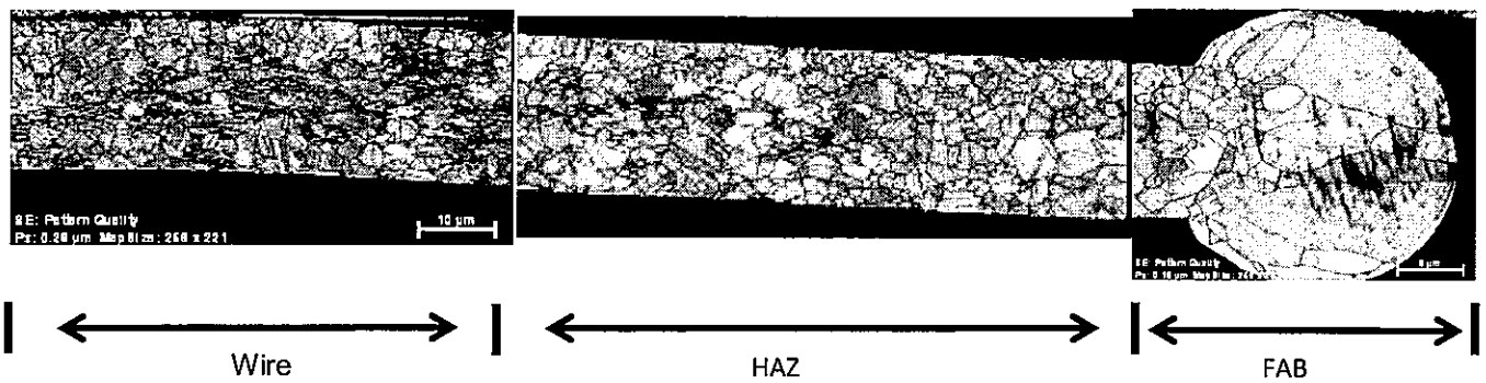
Fig.2 Ion-milled cross-section image wire/HAZ/FAB of wire sample 1
