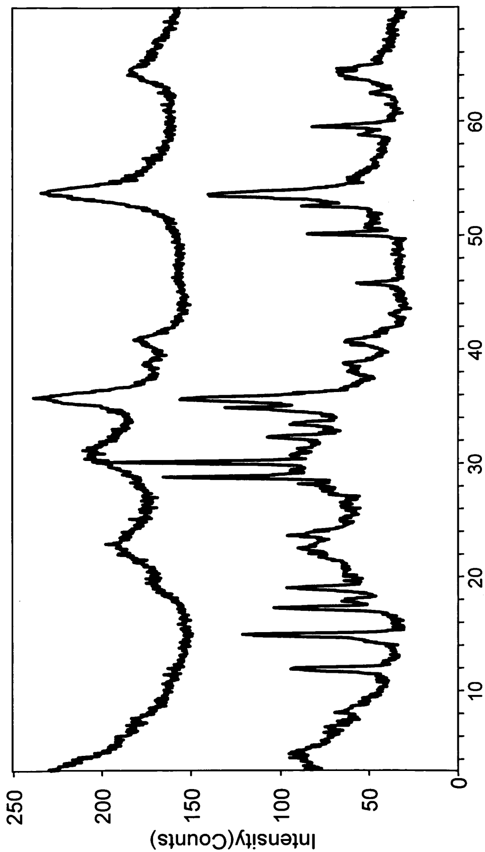
Two-Theta – FIGURE 2
