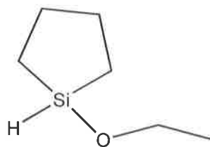
1-ethoxy-1-silacyclopentane
