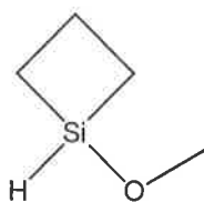
1-methoxy-1-silacyclobutane
