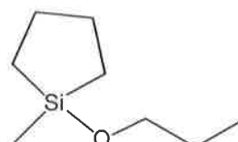
1-methyl-1-n-propoxy-1-silacyclopentane
