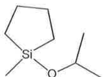
1-methyl-1-iso-propoxy-1-silacyclopentane
