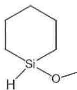
1-methyl-1-methoxy-1-silacyclohexane
