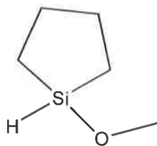
1-methoxy-1-silacyclopentane
