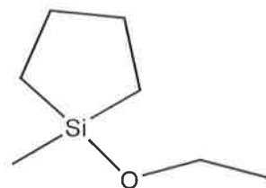
1-methyl-1-ethoxy-1-silacyclopentane
