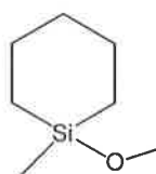
1-methyl-1-methoxy-1-silacyclohexane
