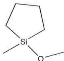
1-methyl-1-methoxy-1-silacyclopentane
