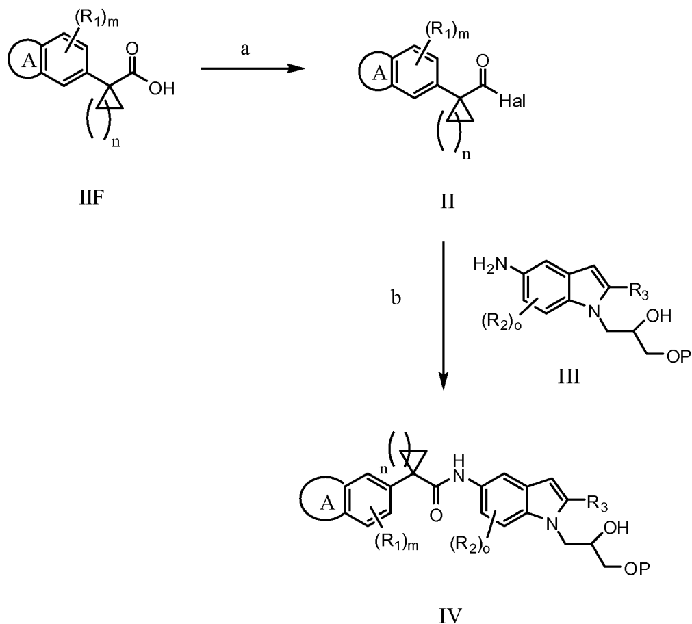
[00138] Scheme 3. Compounds of Formula IV.
