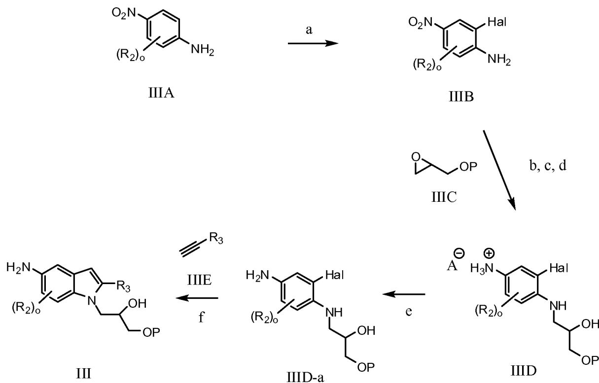
[00131] Scheme 2. Compounds of formula III.
