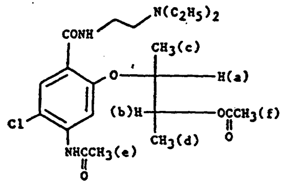
threo isomer
