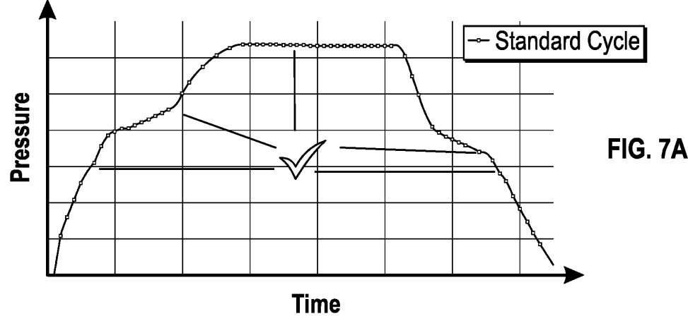
Validation of Correct Open Pressure Applied
