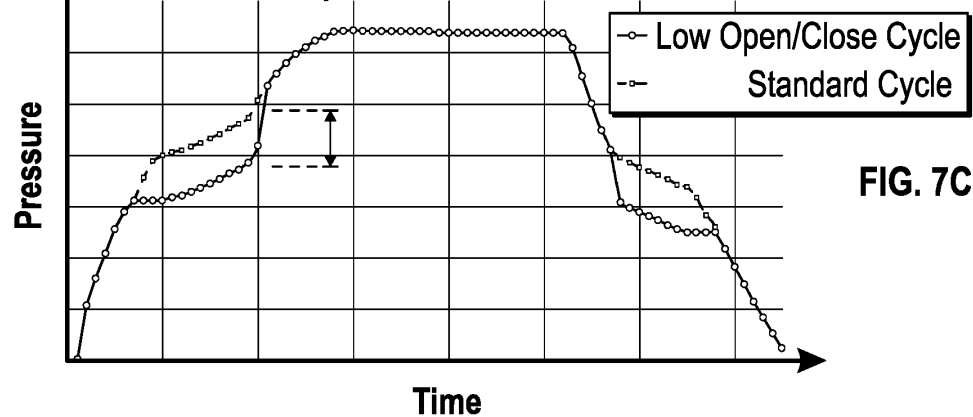
Identification of Non-Standard Cycle - Low Open/Close Pressures
