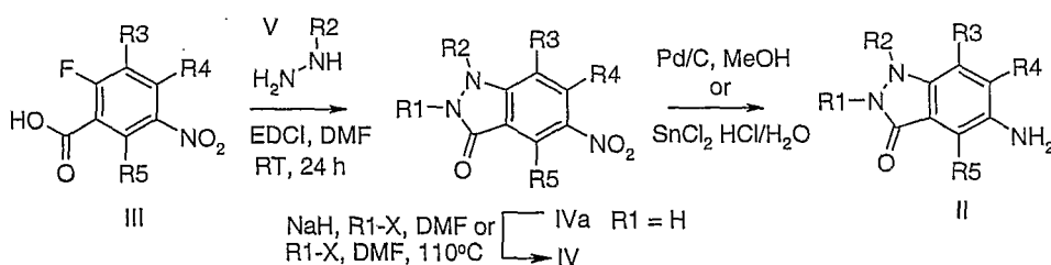
Scheme 3:
