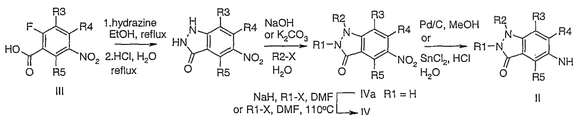
Scheme 2:
