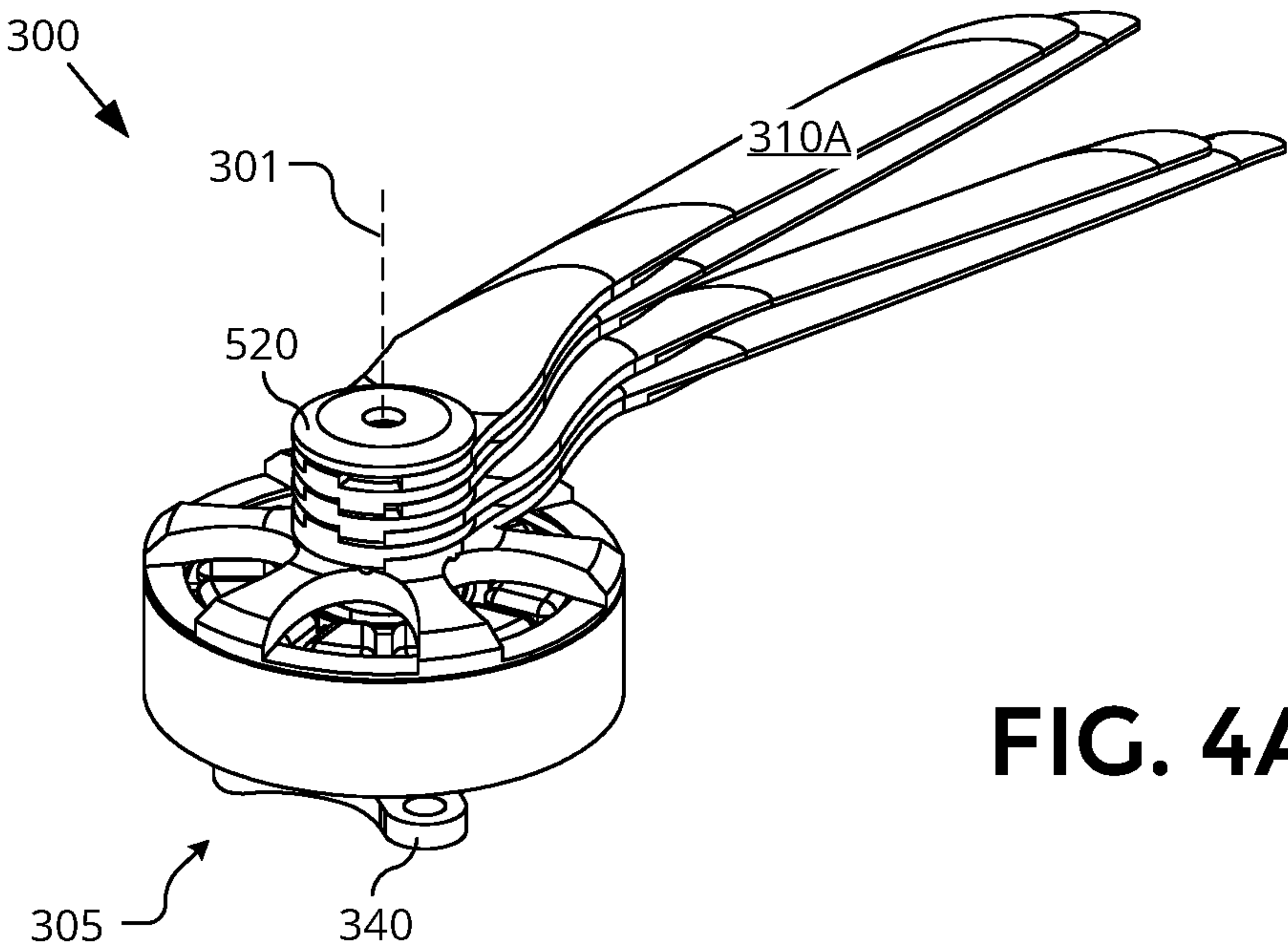
STOWED POSITION (FOLDED PROPELLER BLADES)
