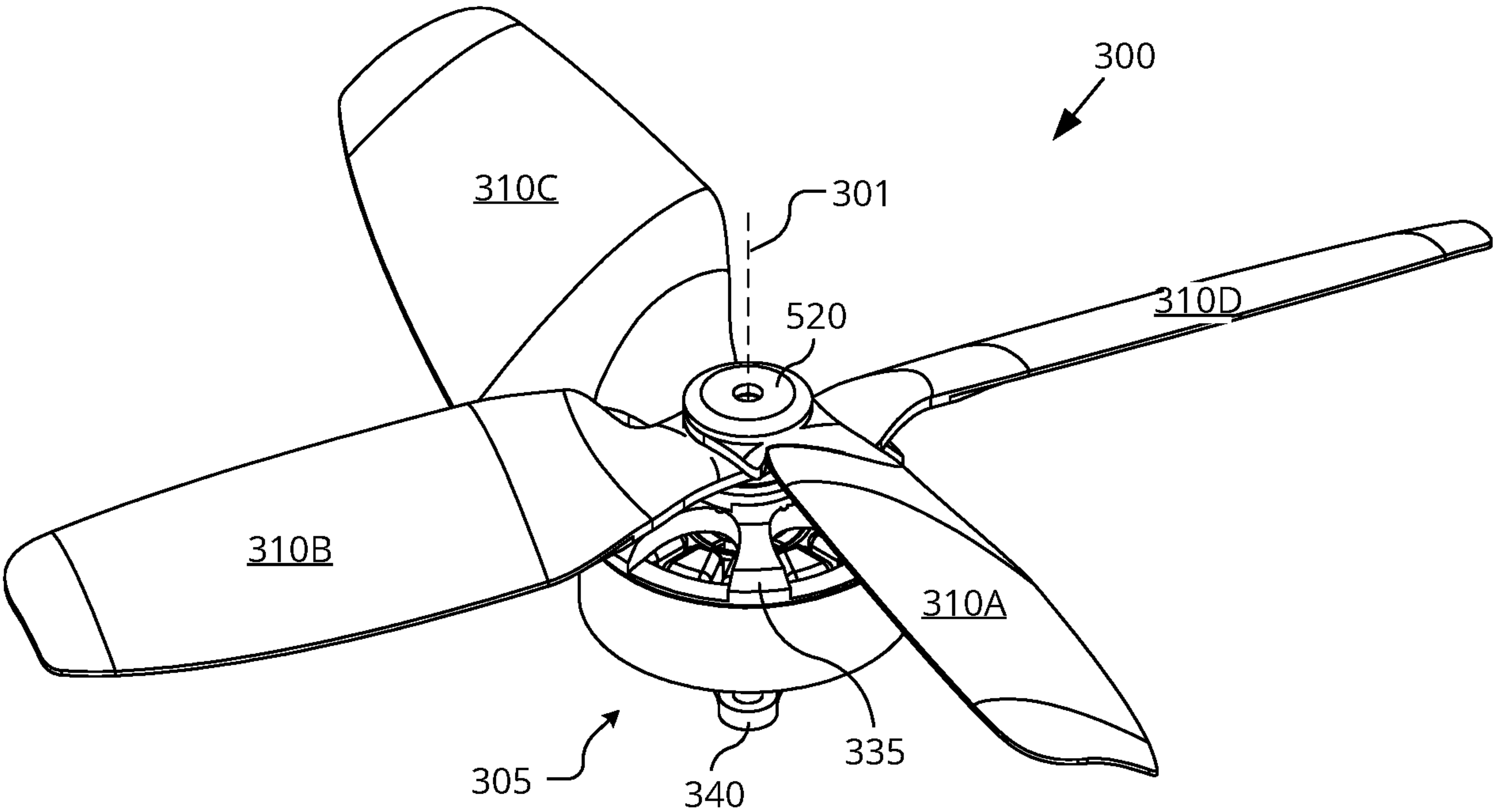
DEPLOYED POSITION (UNFOLDED PROPELLER BLADES)
