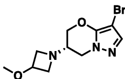
Step 2 – Synthesis of (S)-3-bromo-6-(3-methoxyazetidin-1-yl)-6,7-dihydro-5H-pyrazolo[5,1-b][1,3]oxazine:
