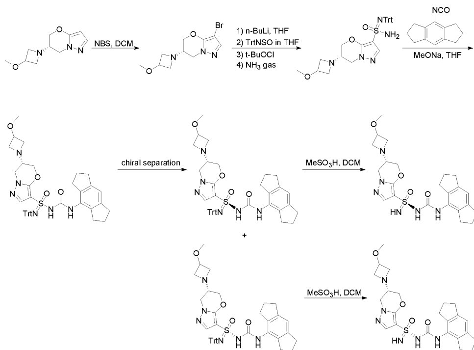
Step 1 – Synthesis of (S)-6-(3-methoxyazetidin-1-yl)-6,7-dihydro-5H-pyrazolo[5,1-b][1,3]oxazine:
