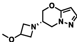
Step 1 – Synthesis of (S)-6-(3-methoxyazetidin-1-yl)-6,7-dihydro-5H-pyrazolo[5,1-b][1,3]oxazine:
