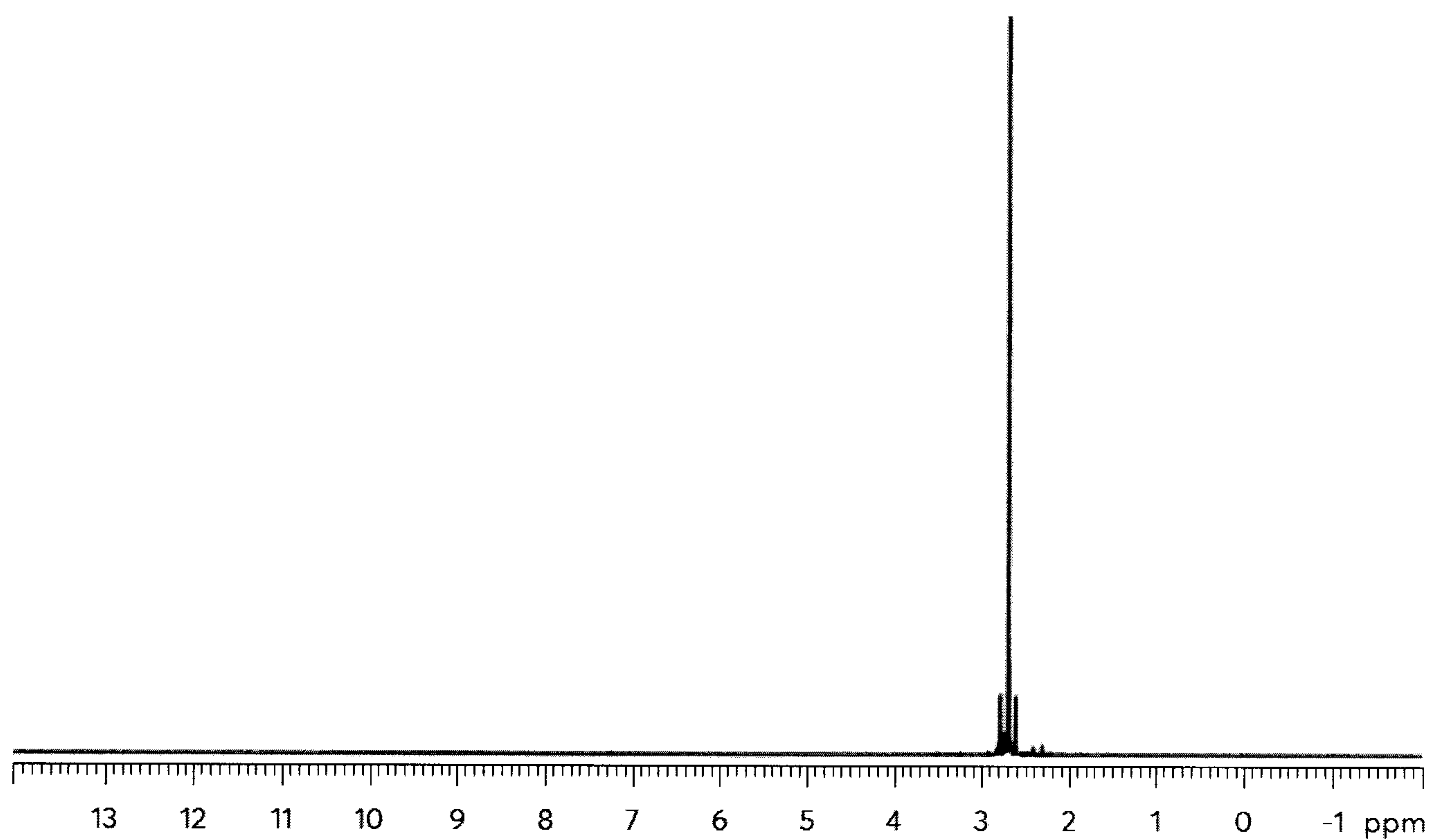
Figure 6: NMR spectrum of Sn(NMe 2 ) 4
