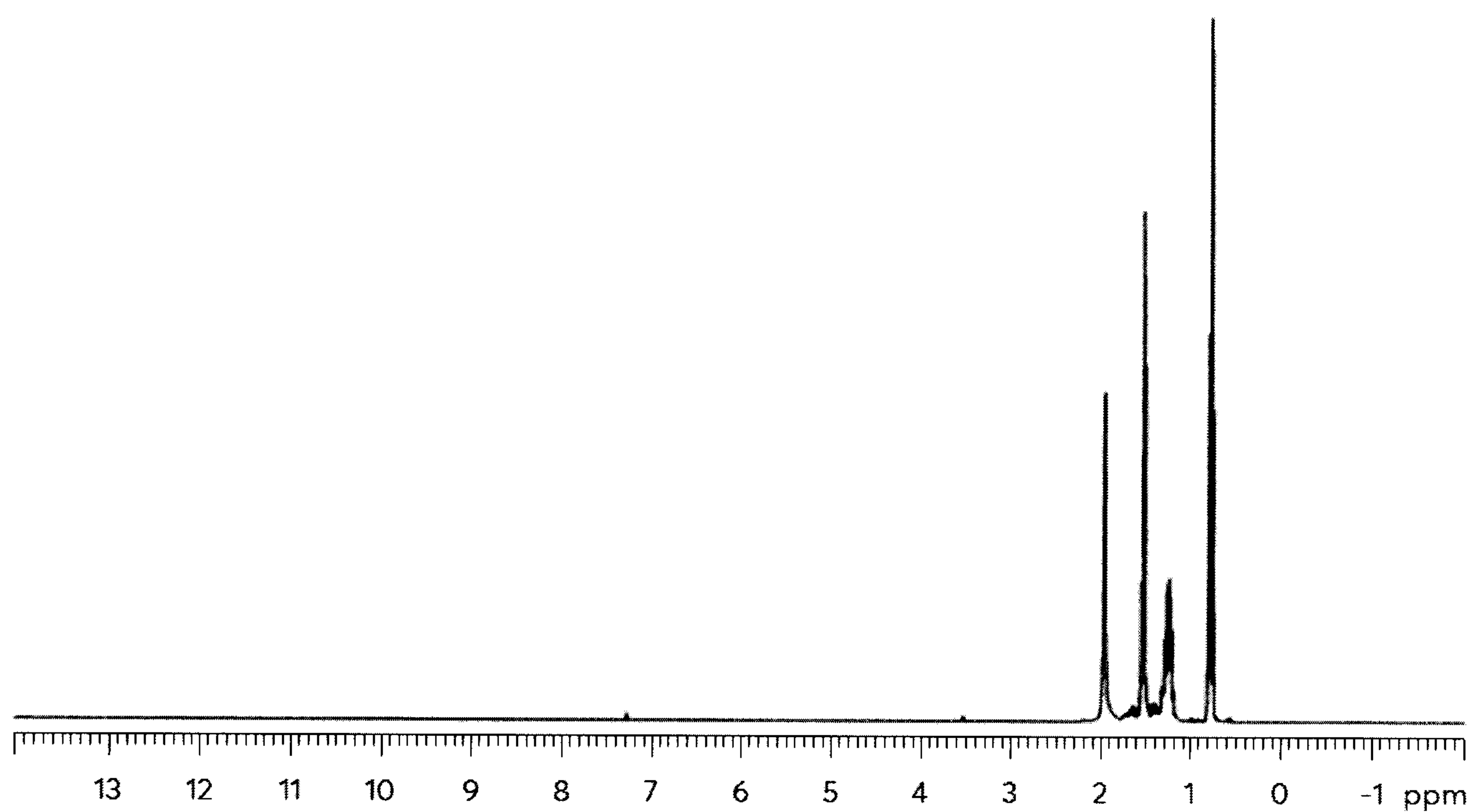
Figure 12: NMR of \text{Bu}_2\text{Sn}(\text{OAc})_2
