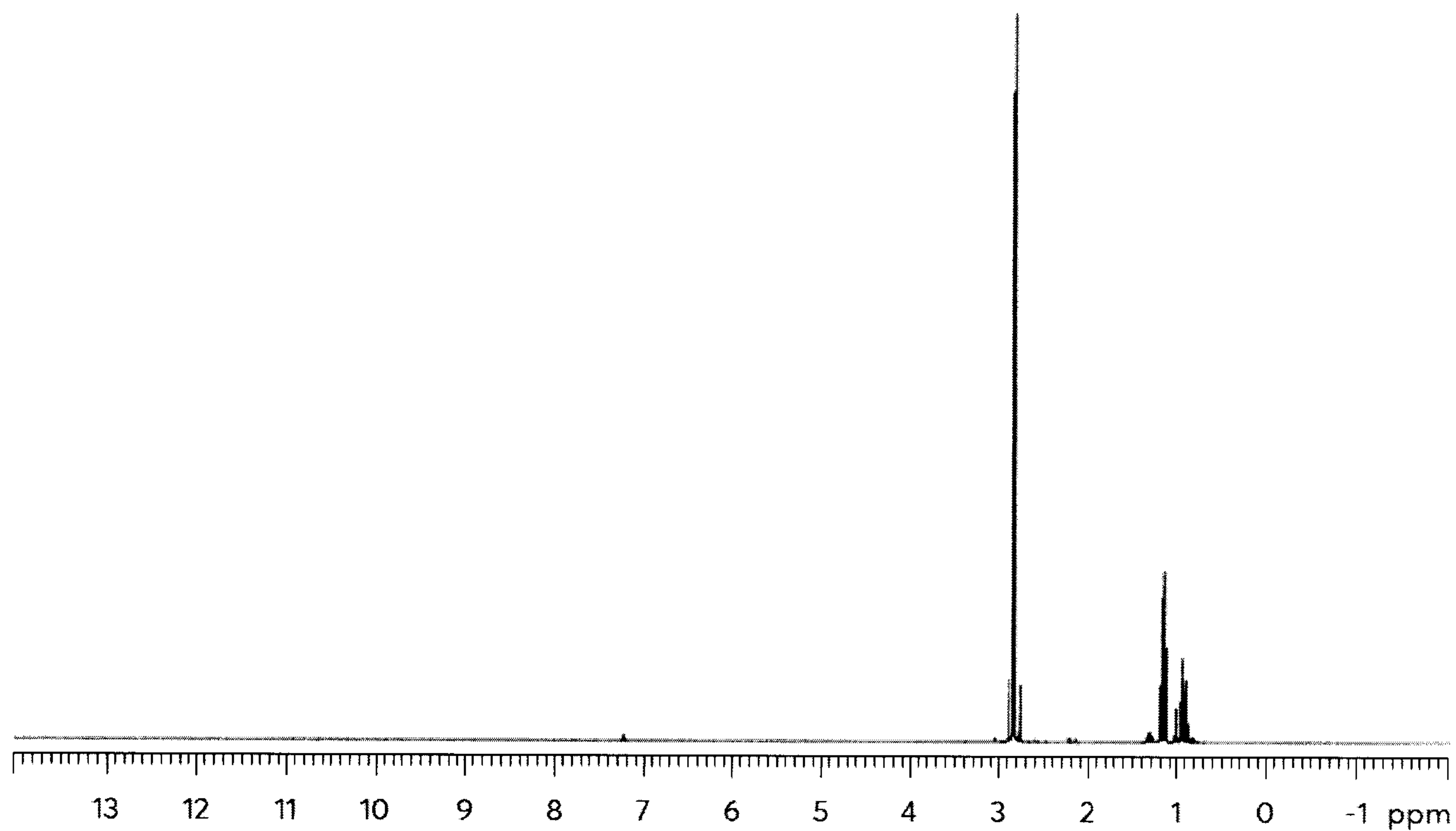
Figure 13: NMR of \text{Et}_2\text{Sn}(\text{NMe}_2)_2
