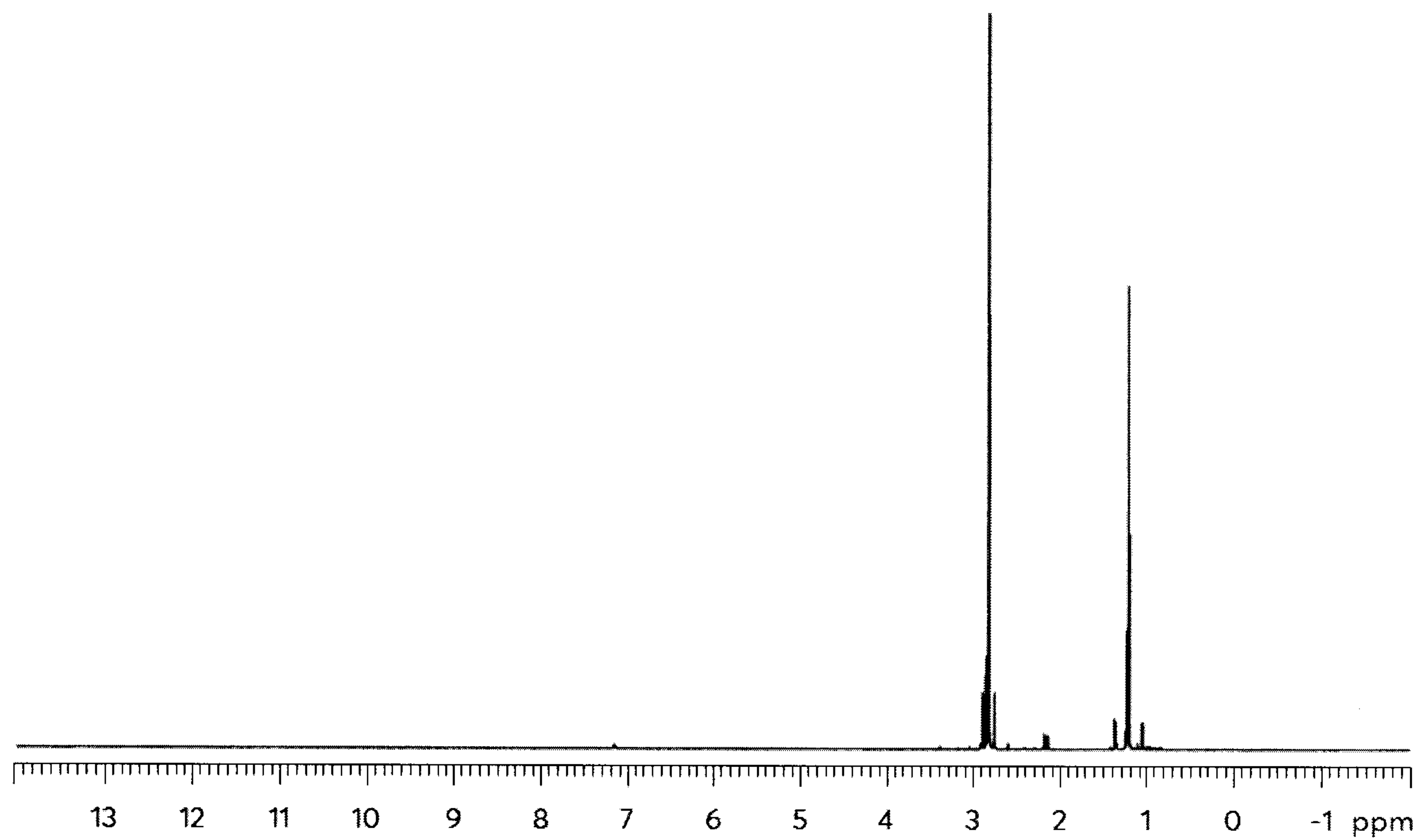
Figure 19: NMR of \text{tBuSn}(\text{NMe}_2)_3
