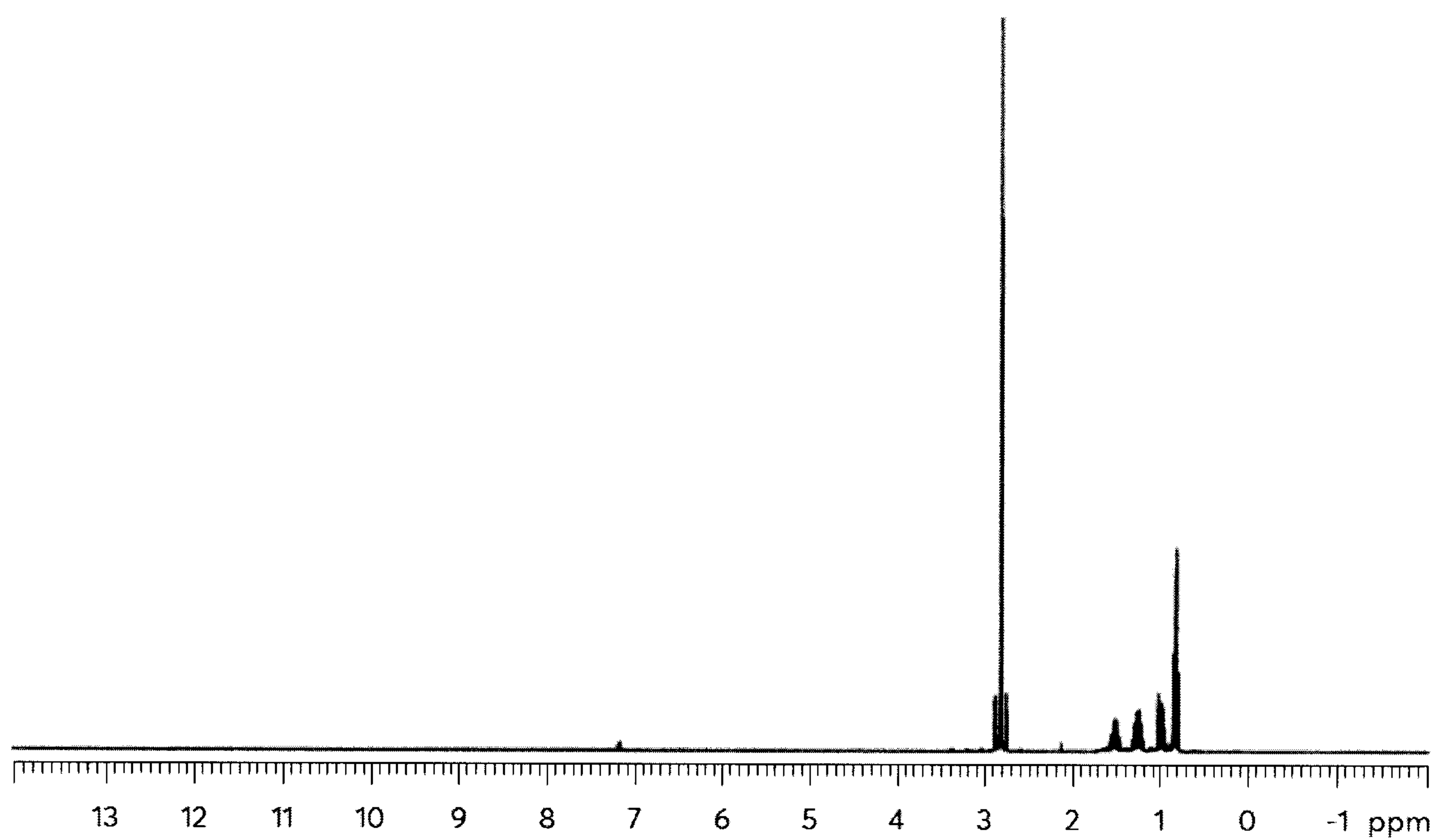
Figure 8: NMR of Bu 2 Sn(NMe 2 ) 2
