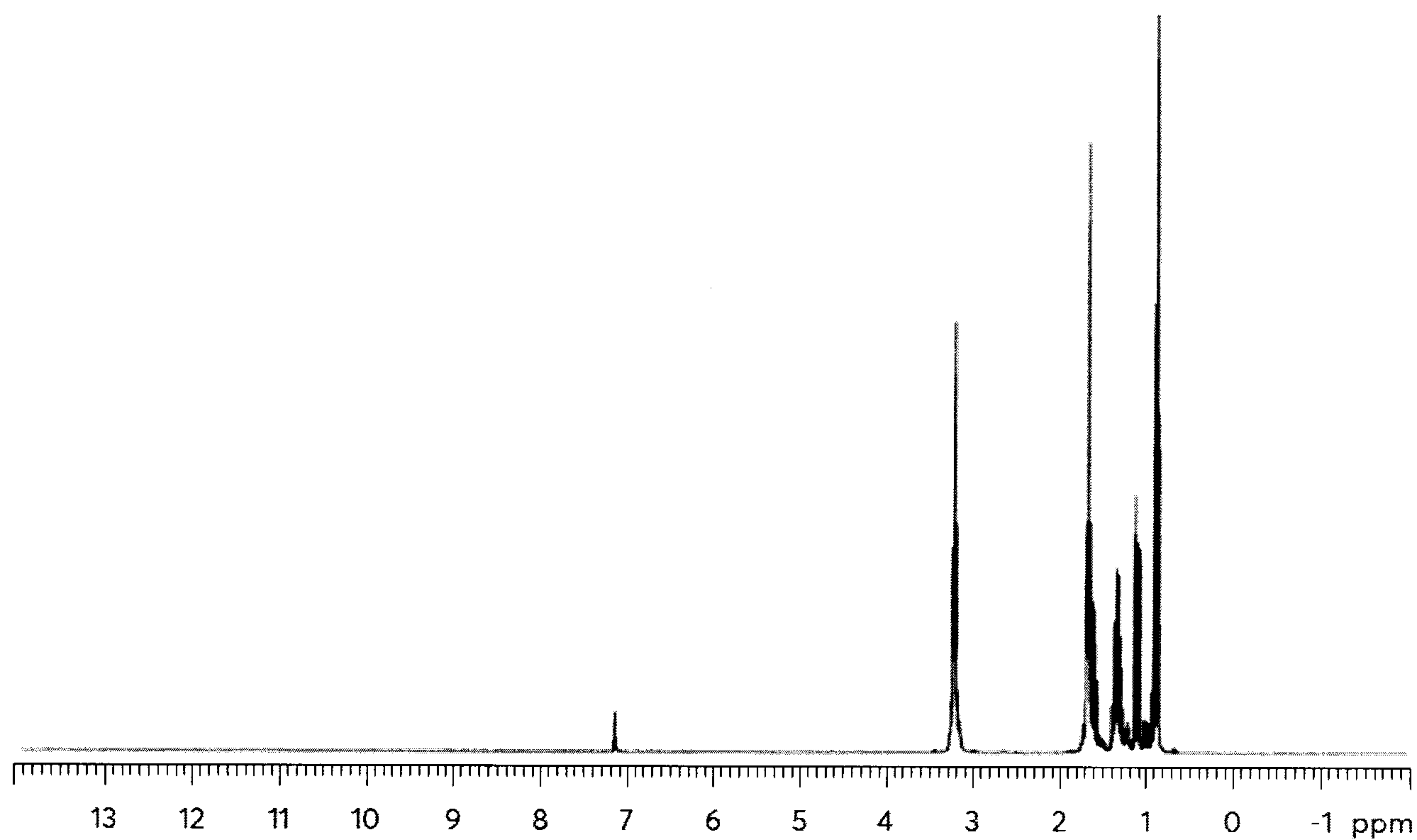
Figure 16: NMR of \text{Bu}_2\text{Sn}(\text{Pyrrolodiny})_2
