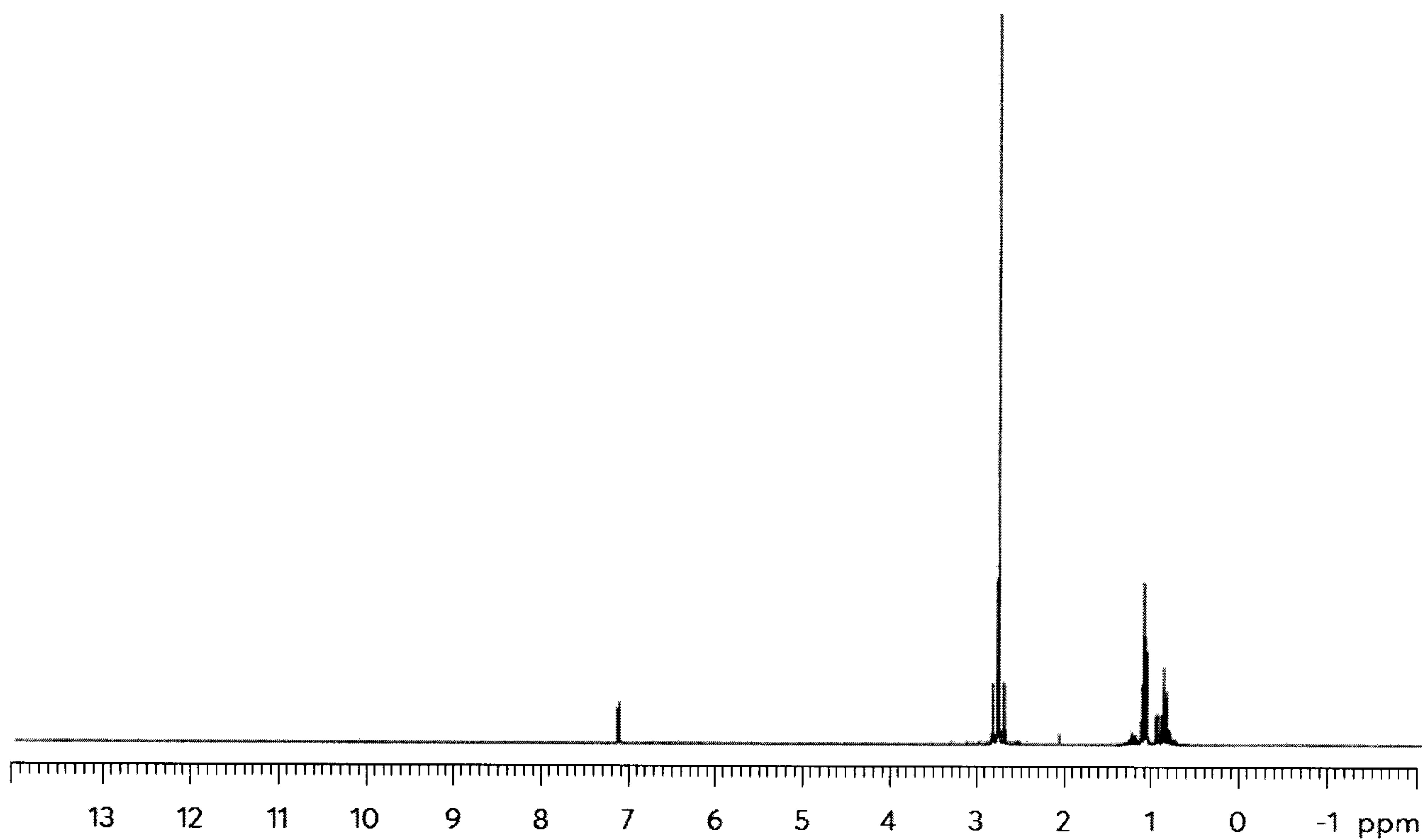
Figure 14: NMR of Me 2 Sn(NEt 2 ) 2
