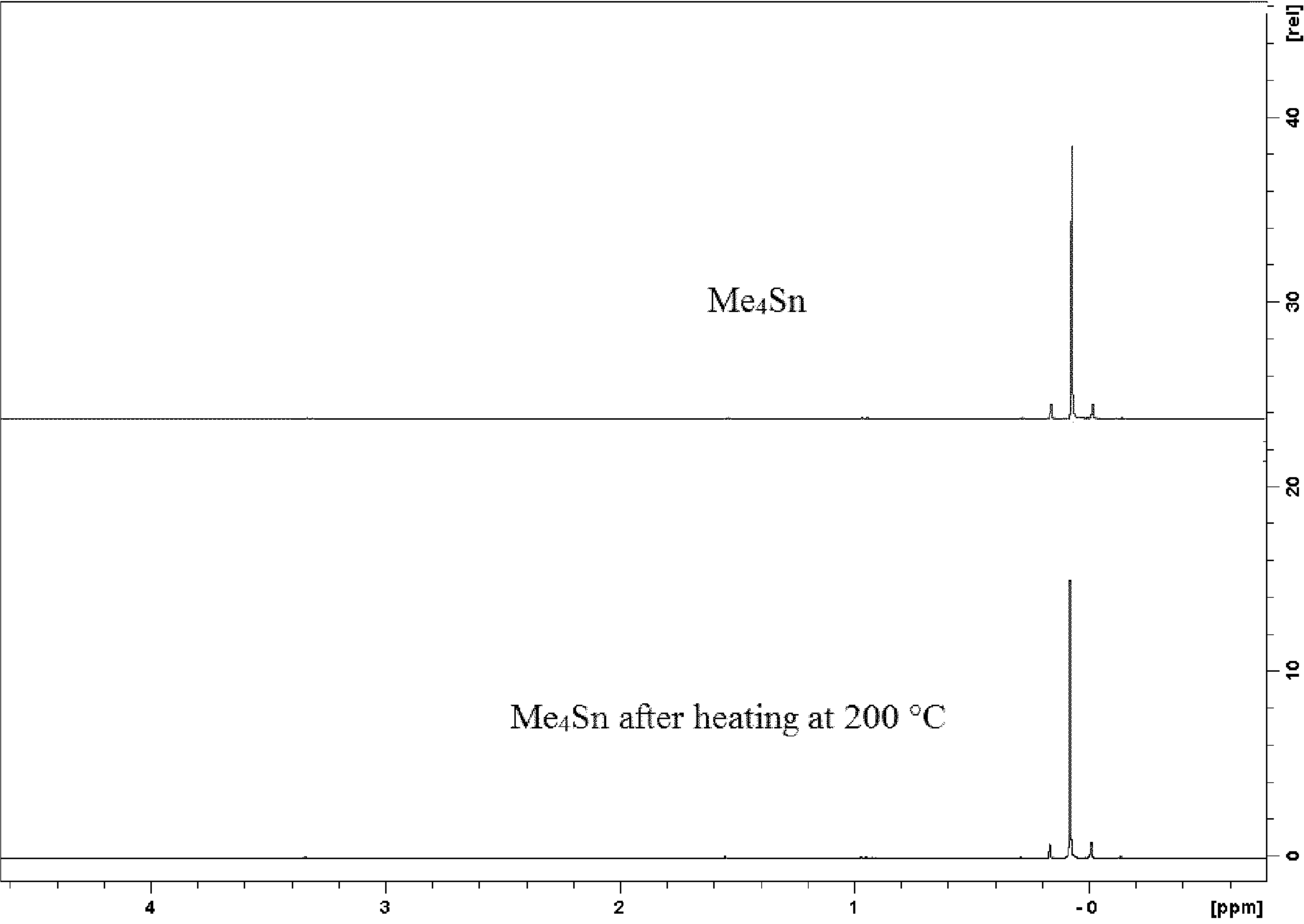
Figure 25. NMR of Me 4 Sn before and after heating at 200 °C
