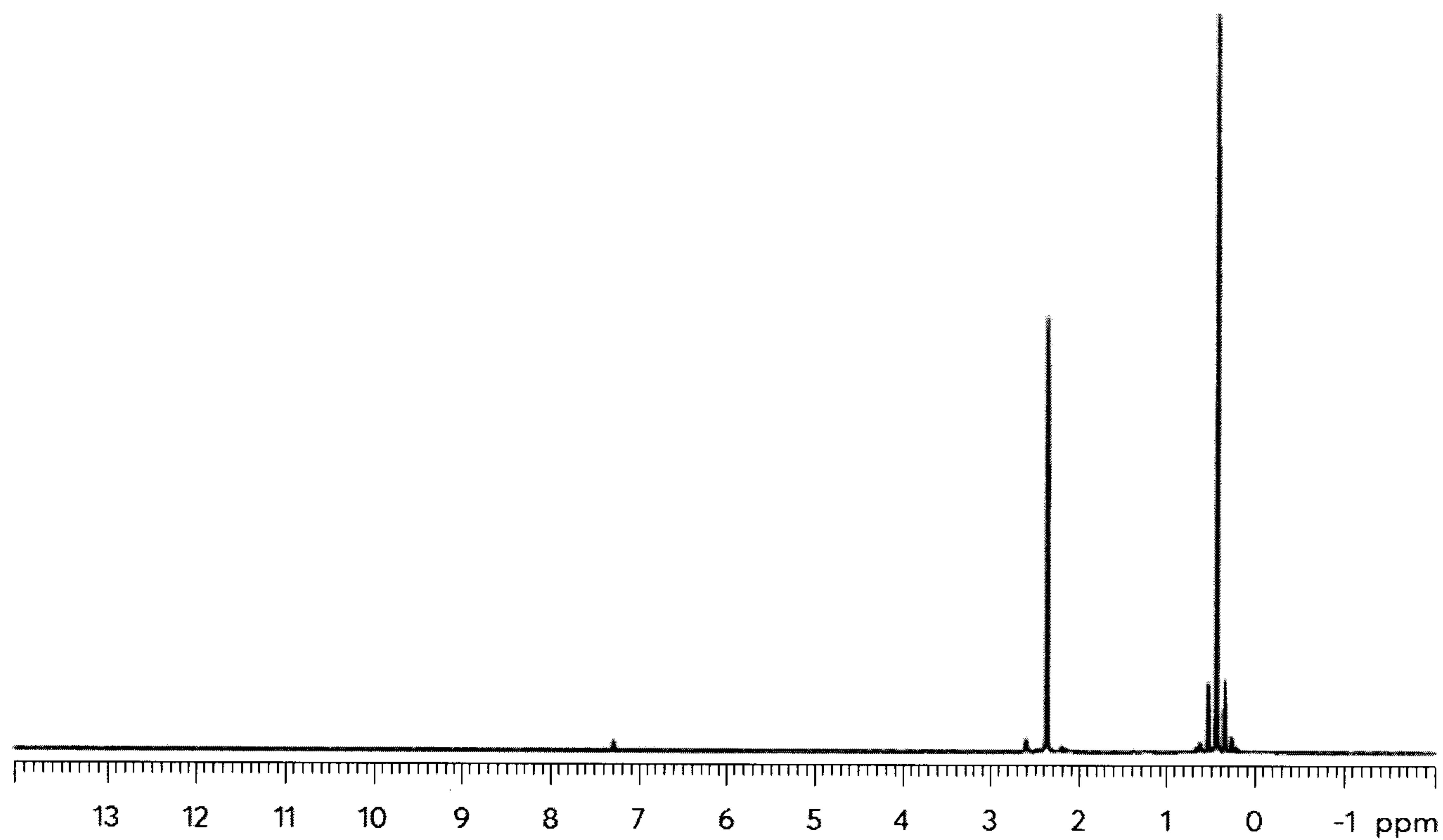
Figure 5: NMR spectrum of Me 3 SnNMe 2
