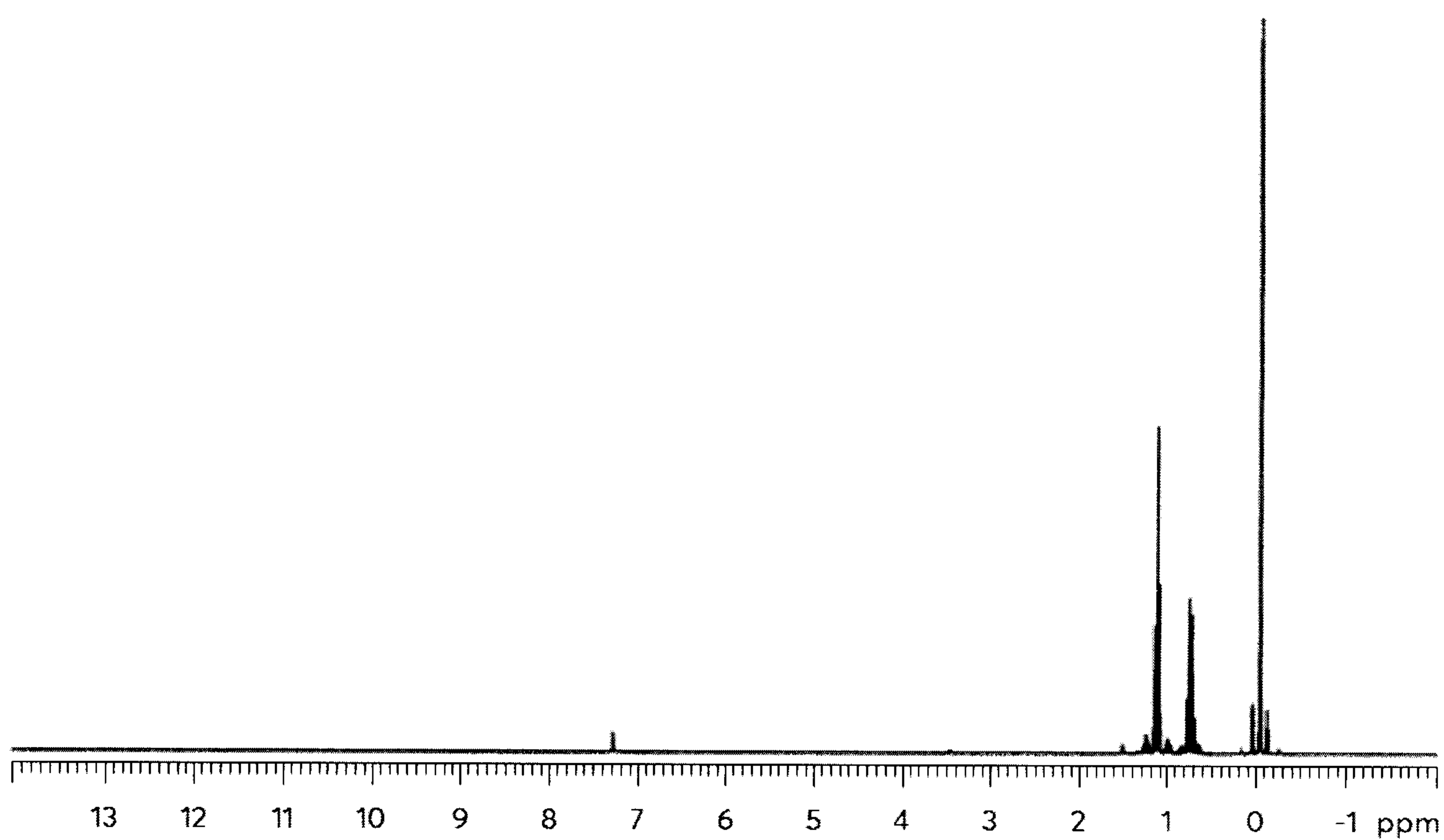
Figure 9: NMR of Me 2 SnEt 2
