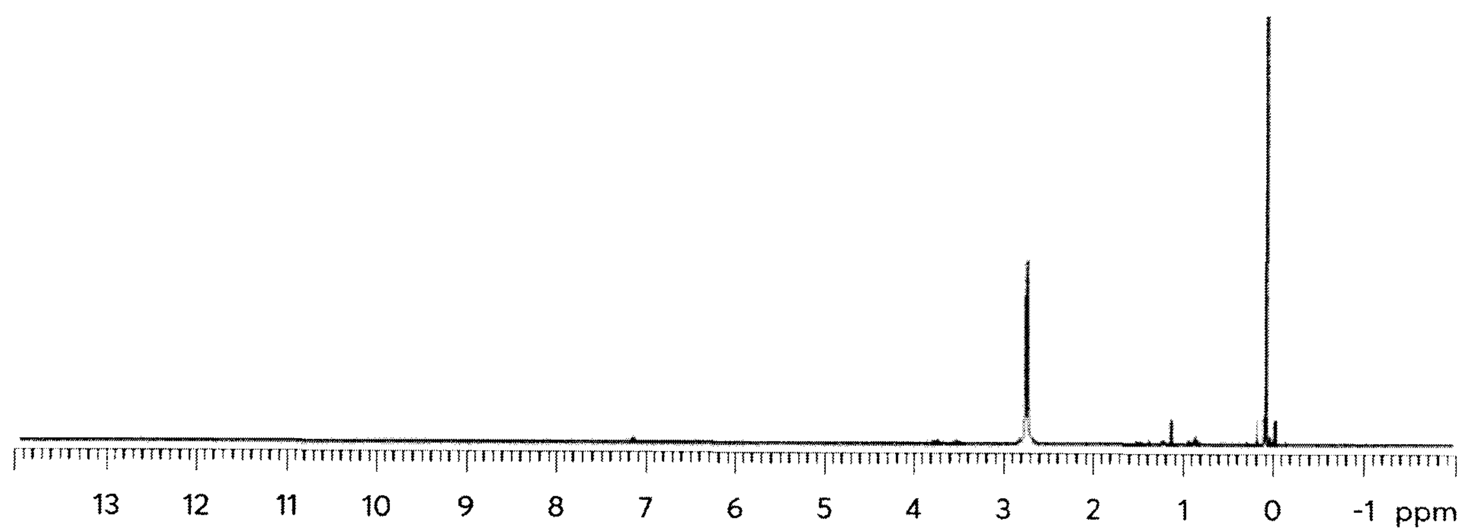
Figure 18: NMR of Me 2 Sn(NMe 2 ) 2
