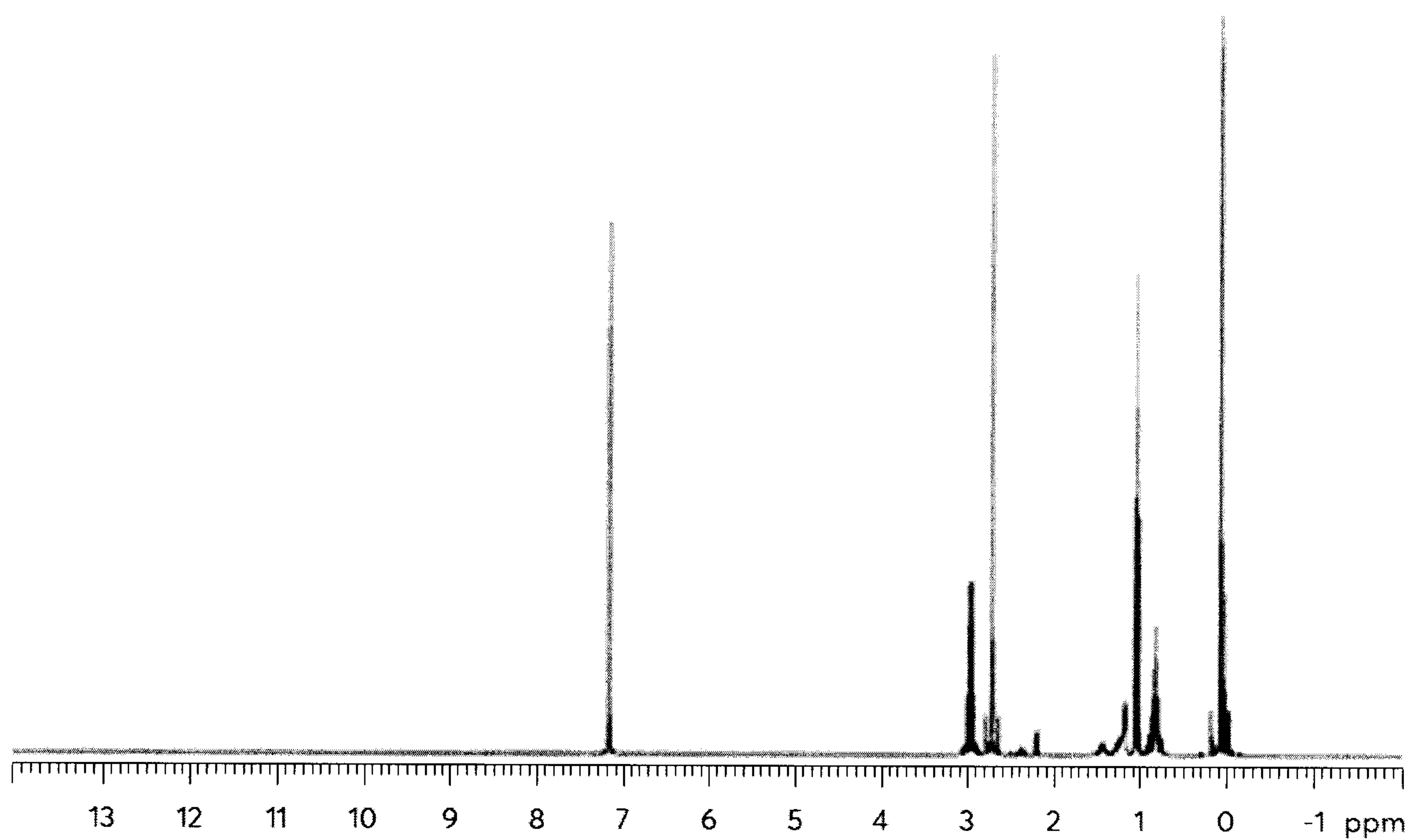
Figure 7: NMR of Me 2 Sn(NEtMe) 2
