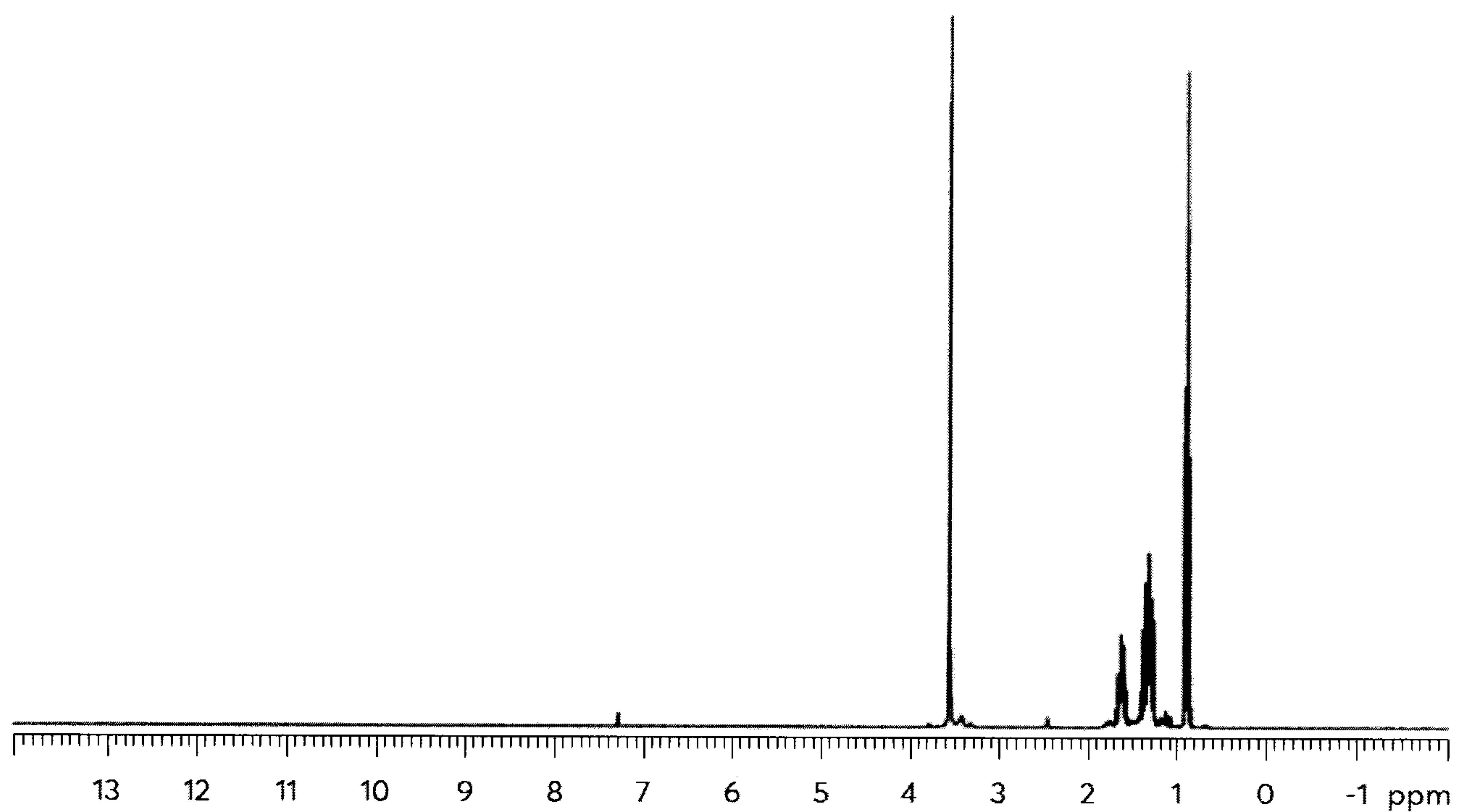
Figure 11: NMR of \text{Bu}_2\text{Sn}(\text{OMe})_2
