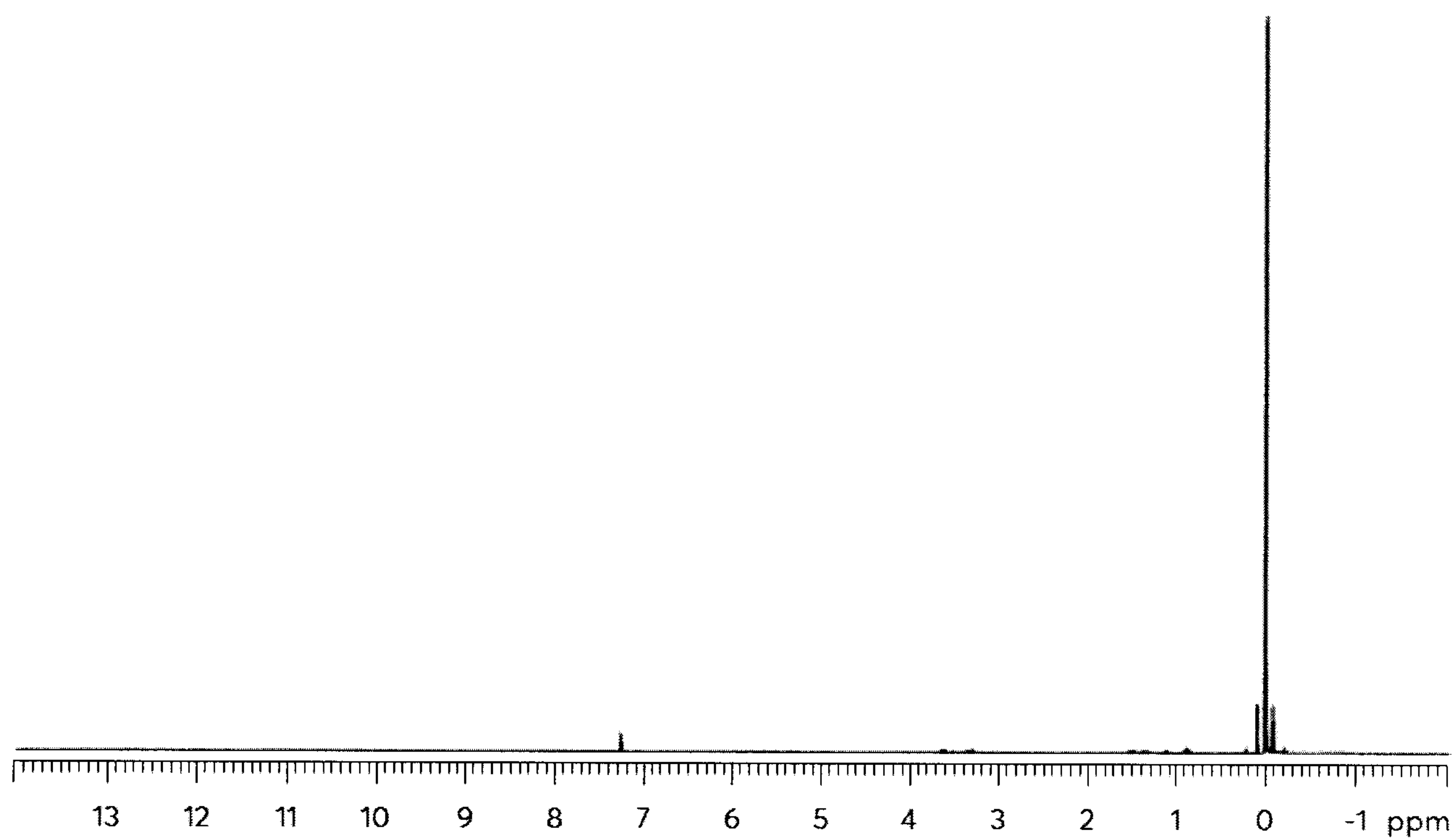
Figure 10: NMR of Me 4 Sn
