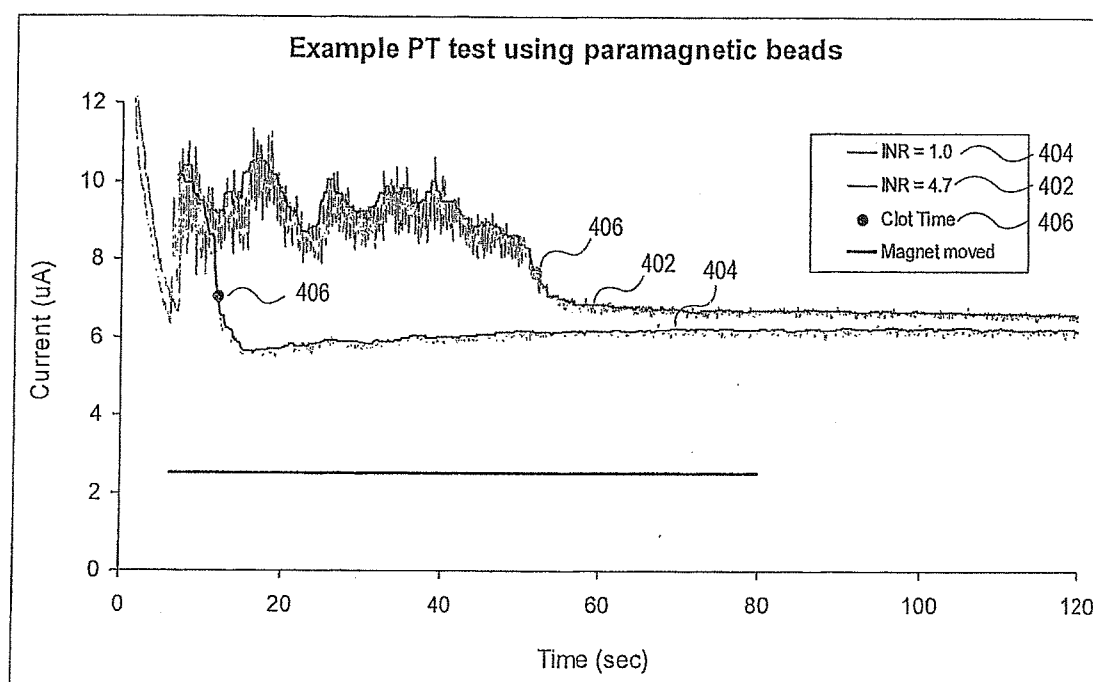
Graph of an exemplary coagulation reaction
