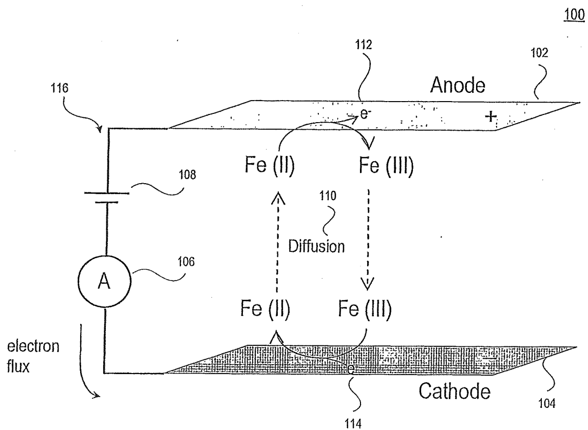
Diagram of an exemplary two-electrode amperometry
