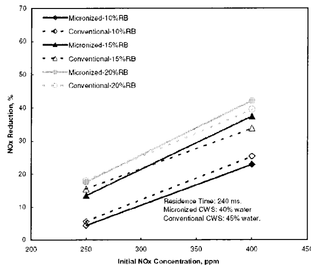
Figure 4-4. NOx reduction as a function of initial NOx concentration at 240 ms residence time.
