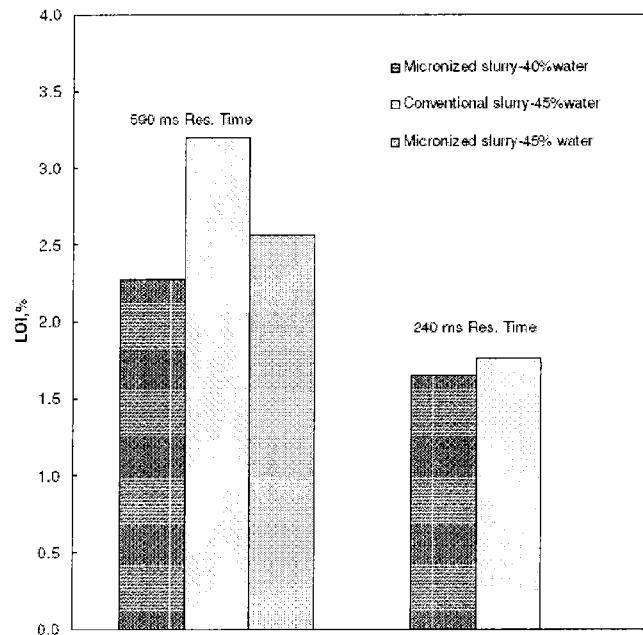
Figure 4-7. Comparison of Loss on Ignition (LOI).
