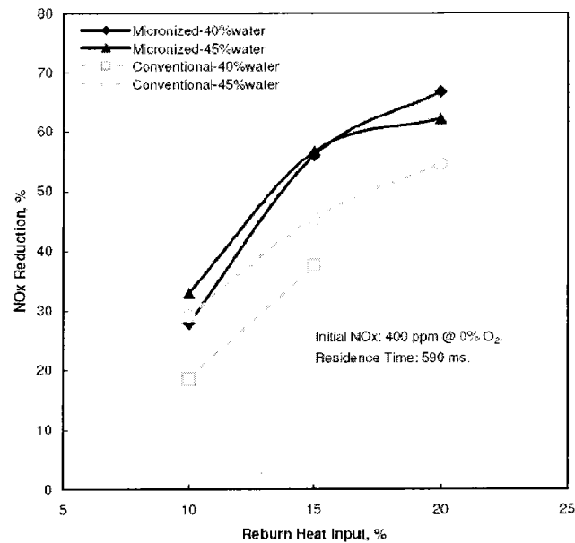
Figure 4-1. NOx reduction (%) at 400 ppm initial NOx and 590 ms residence time.
