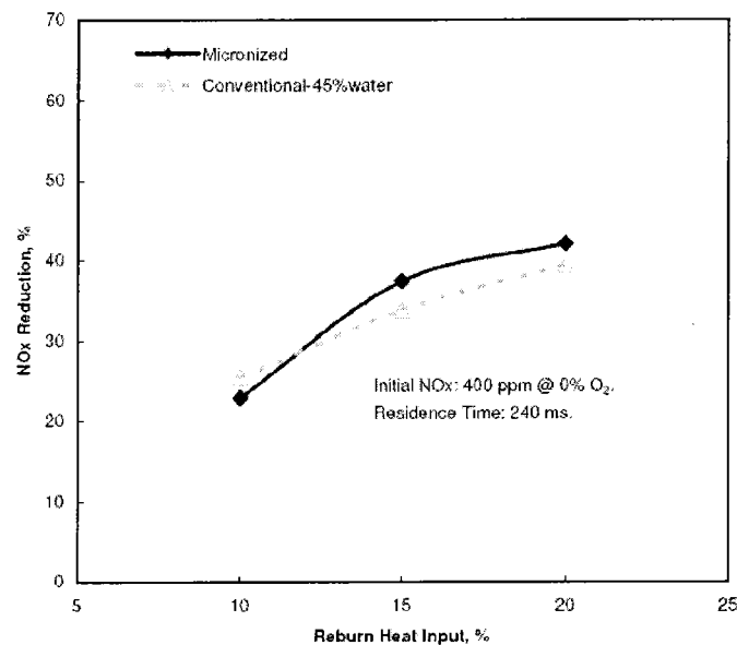
Figure 4-2. NOx reduction (%) at 400 ppm initial NOx and 240 ms residence time.
