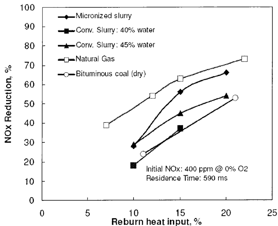
Figure 4-6. Comparison of slurry reburn performance vs. other fuels
