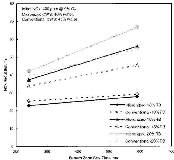
Figure 4-5. NO x reduction as a function of reburn zone residence time at 400 ppm initial NO x .
