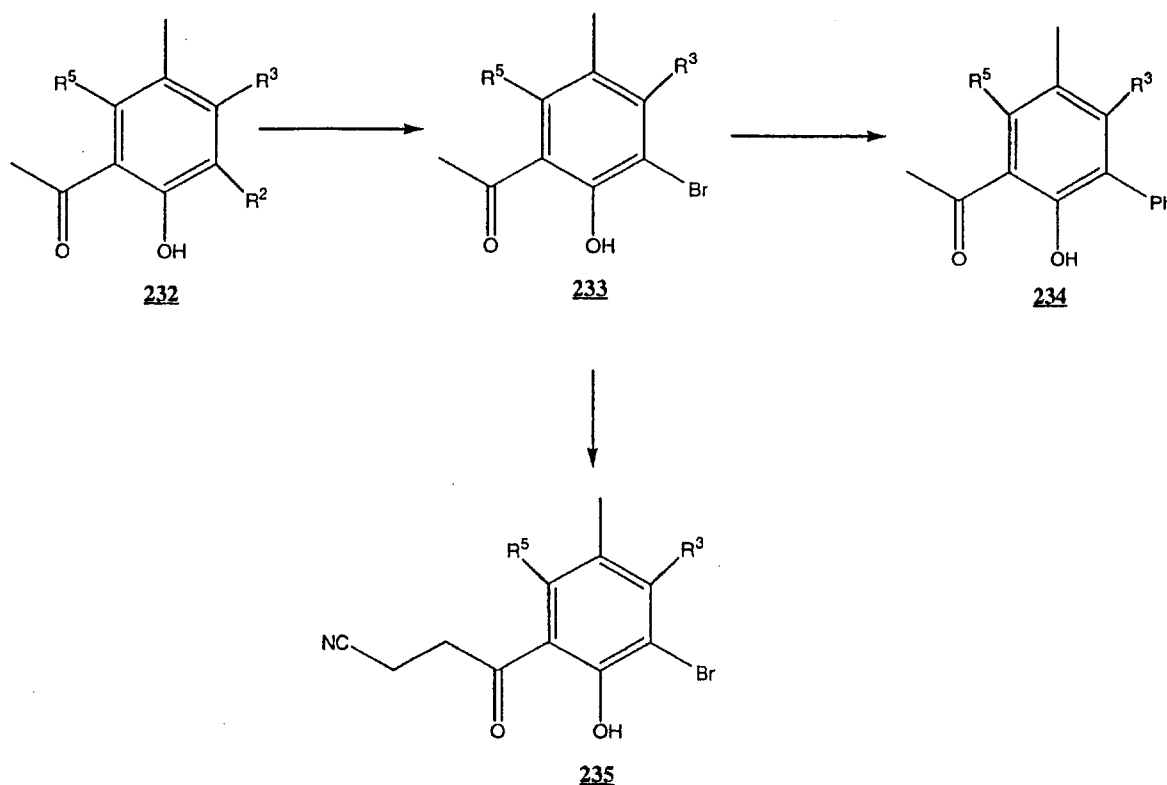
Scheme LVIII
