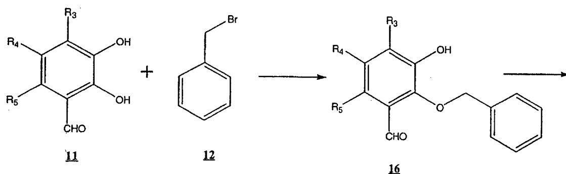
Scheme VII
