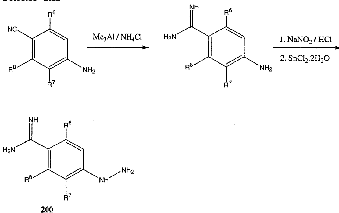
Scheme LXI
