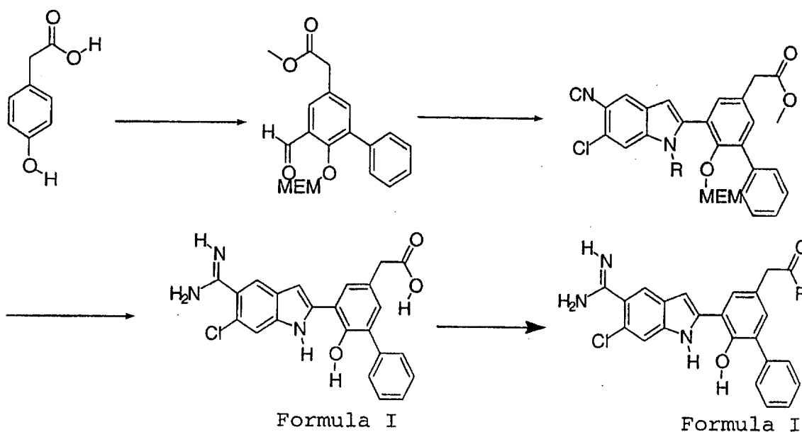
Scheme LXXI
