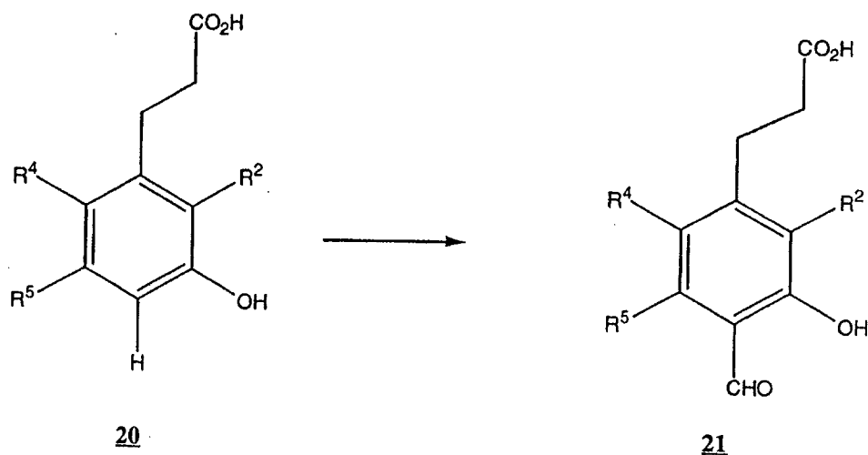
Scheme IX
