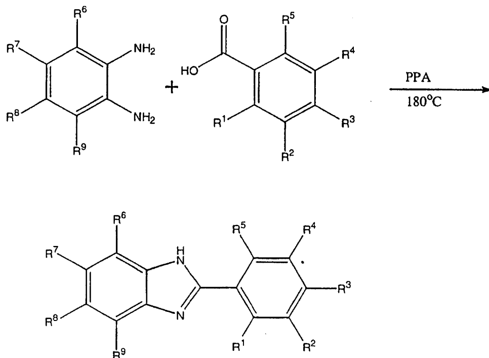
Formula I
