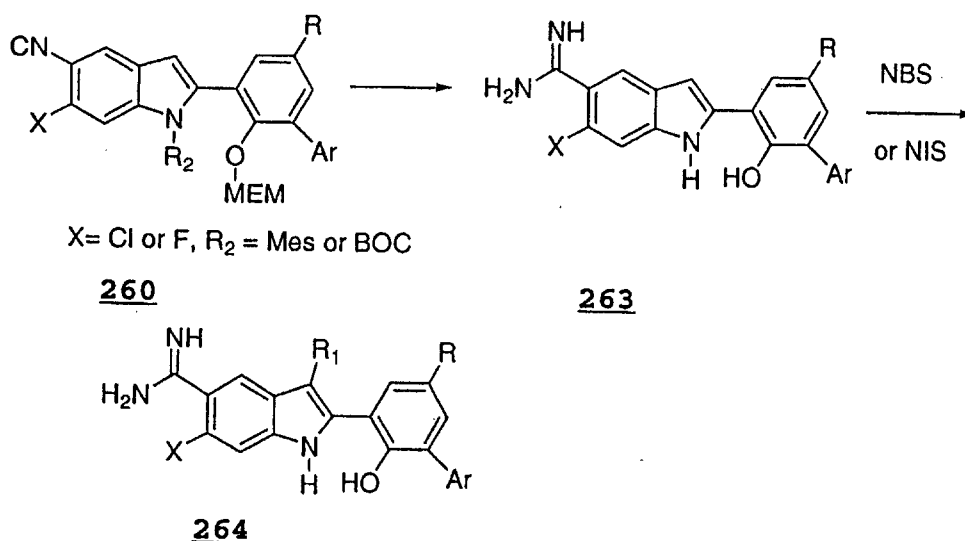
Scheme LXXIII
