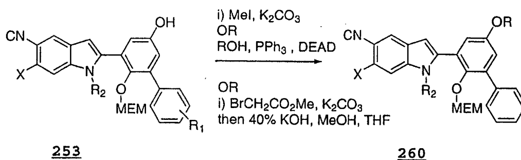
Scheme LXX
