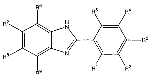
Formula Ia
