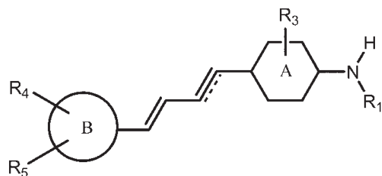
Formula (I-ii)
