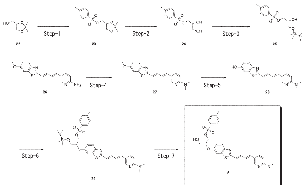
Synthesis scheme
