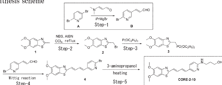
Synthesis scheme
