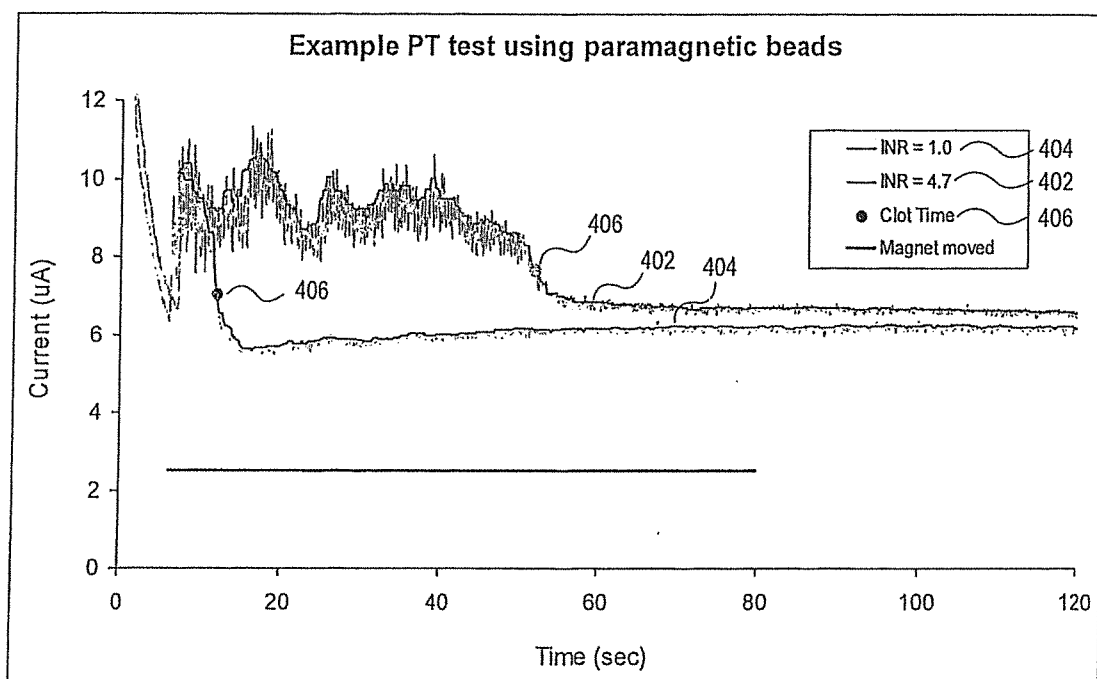
Graph of an exemplary coagulation reaction
