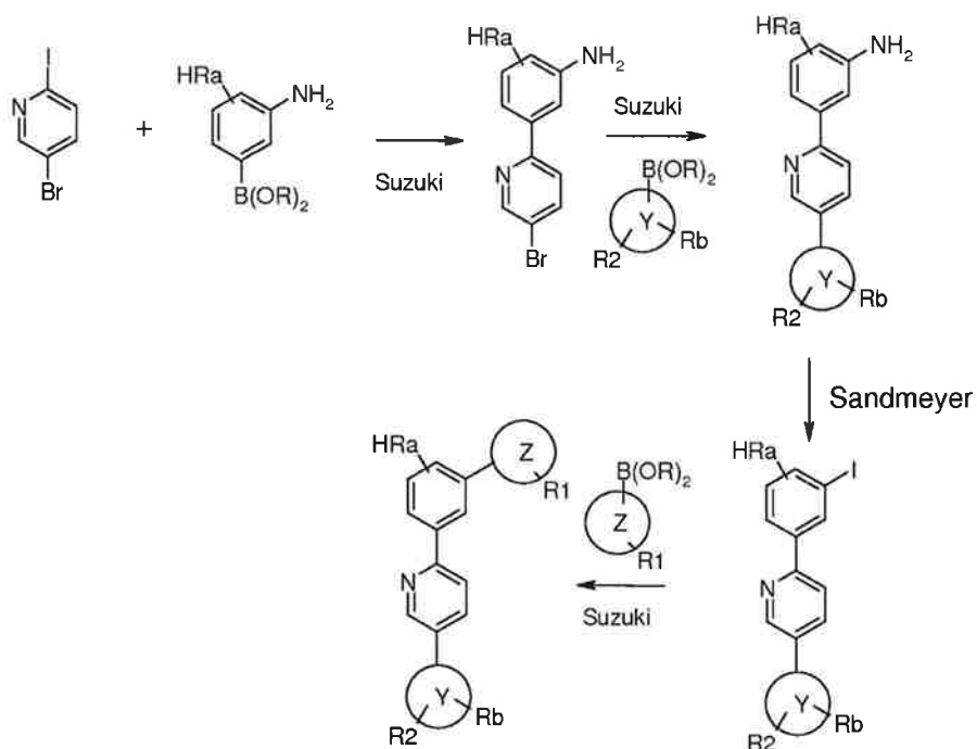
Scheme 2: Example of synthetic route for pyridinyl-pyridines
