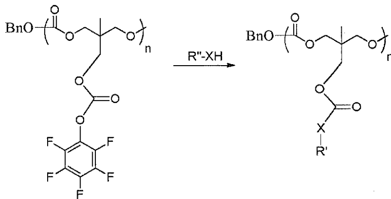
Scheme 8.
