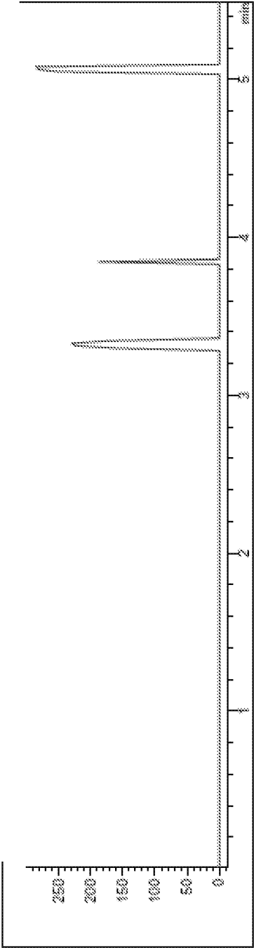
Figure 4: Typical Chromatogram of compound 1.
