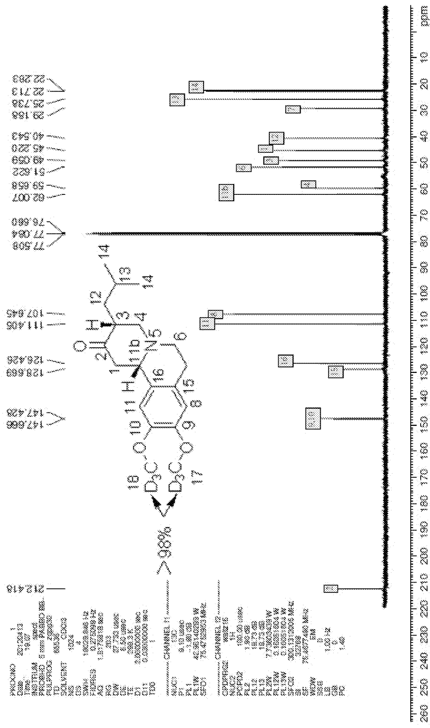
Figure 3: 13 C NMR of compound 1
