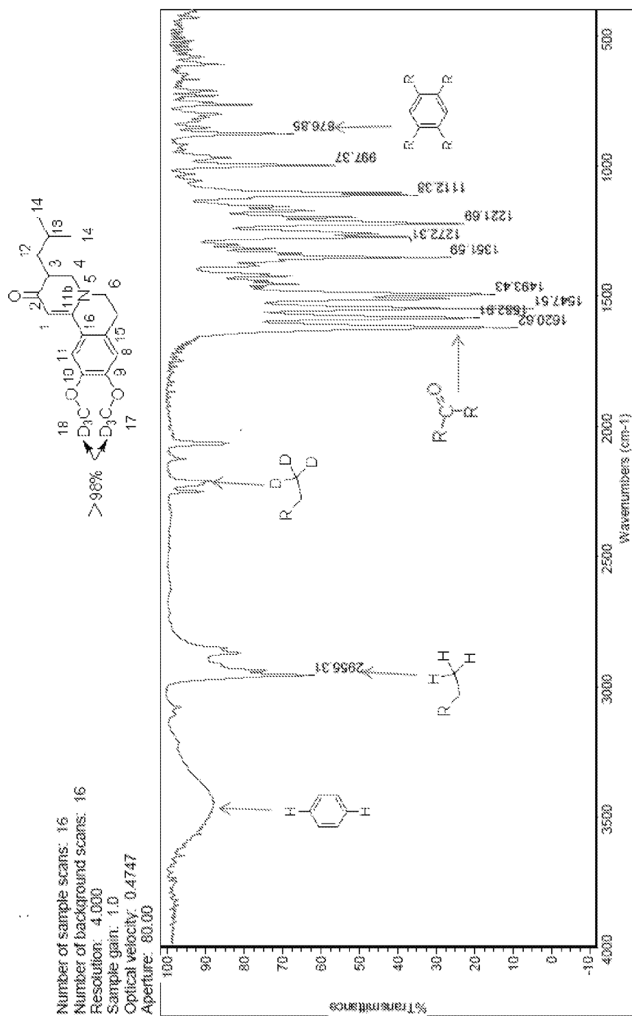
Figure 5: FTIR Spectra of compound 2.
