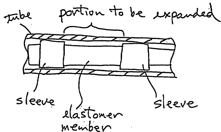
Fig. D : Schematic view of FR-A-2220326 (D3)
