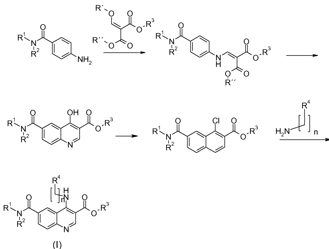
Reaction Scheme 1
