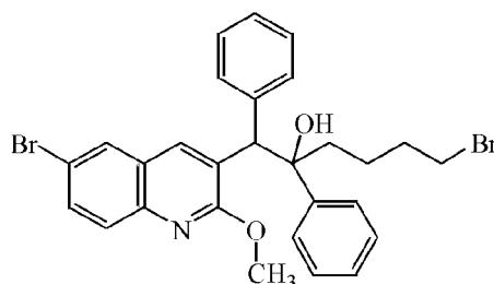
Intermediate 39 (mixture of diastereoisomers)
