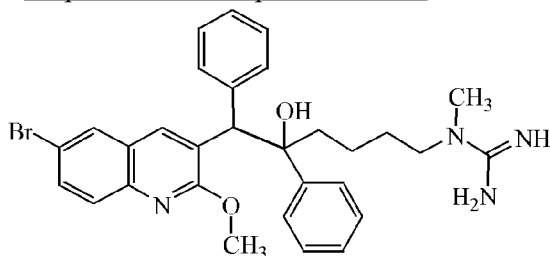
Compound 1 (dia A)
