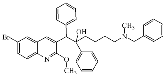
Intermediate 2 (dia A) Intermediate 3 (dia B)
