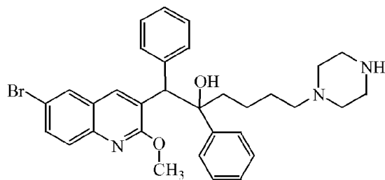
Intermediate 8 (dia A)
