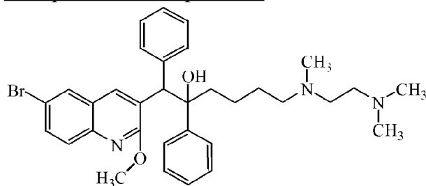
Compound 51 (dia B)
