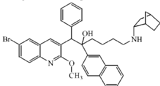
Compound 38 (dia A; endo) Compound 39 (B1; endo) Compound 40 (B2; endo)
