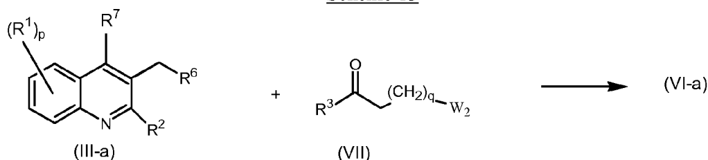
Scheme 13
