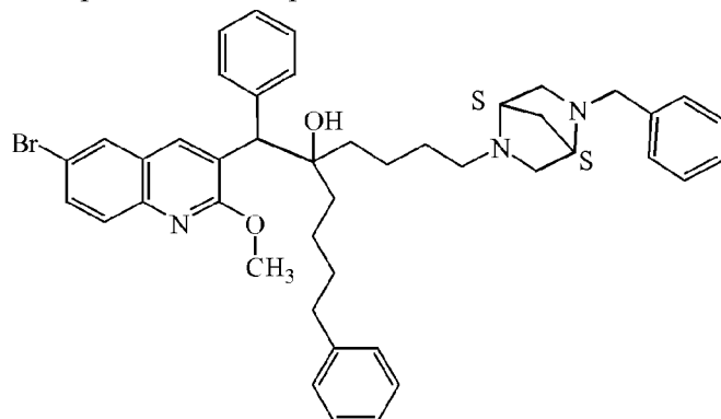
Compound 16 (dia A) Compound 17 (dia B)
