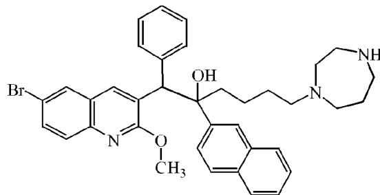
Compound 33 (dia B)
