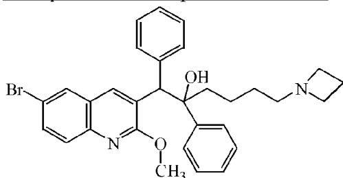
Compound 41 (dia B)
