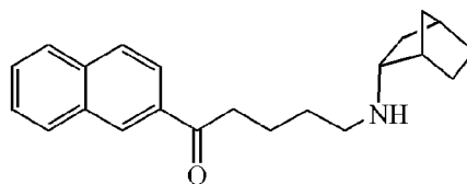
Intermediate 38 (endo)
