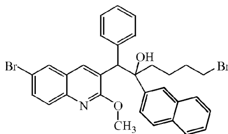
Intermediate 48 (mixture of diastereoisomers)
