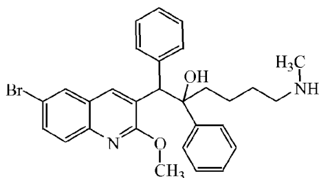
Intermediate 4 (dia A)
