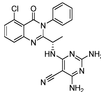
Compound Z
