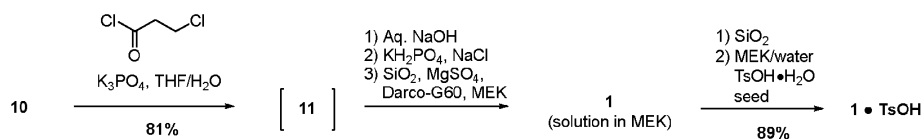
Scheme 4. Second Alternate Preparation of 1
