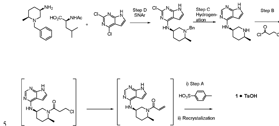
Scheme 4. Second Alternate Preparation of 1
