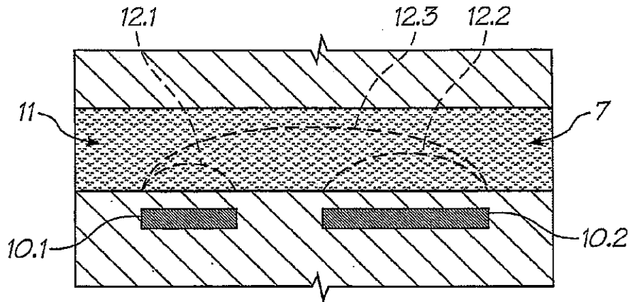
FIG. 52 (PRIOR ART)
