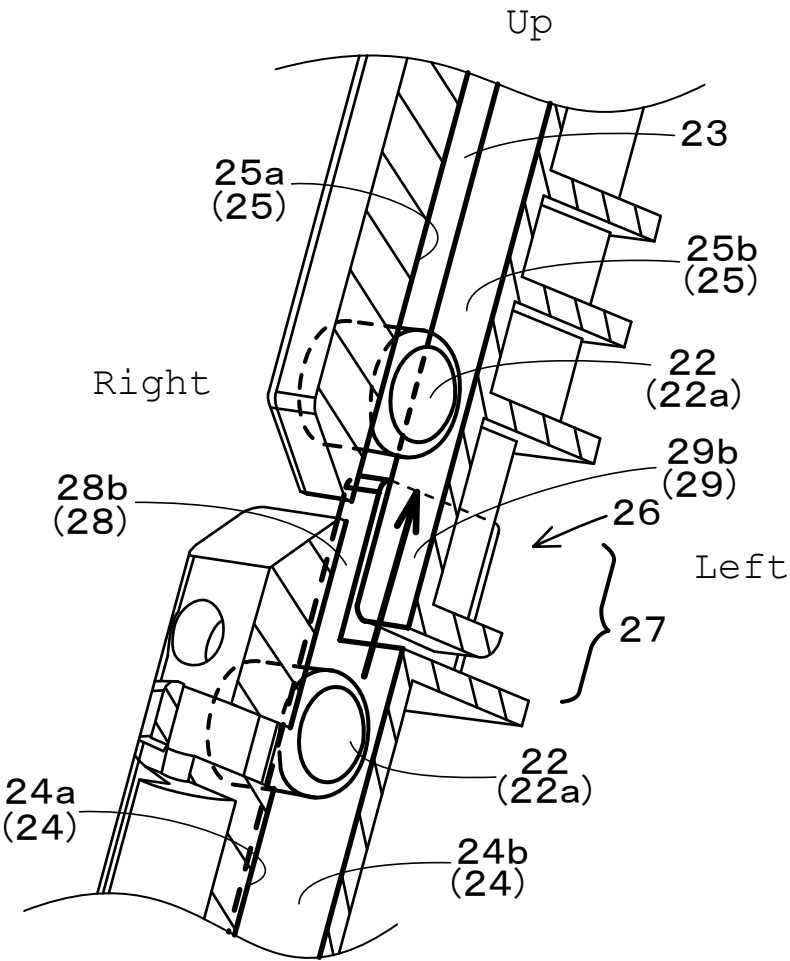
Enlargement of C part
