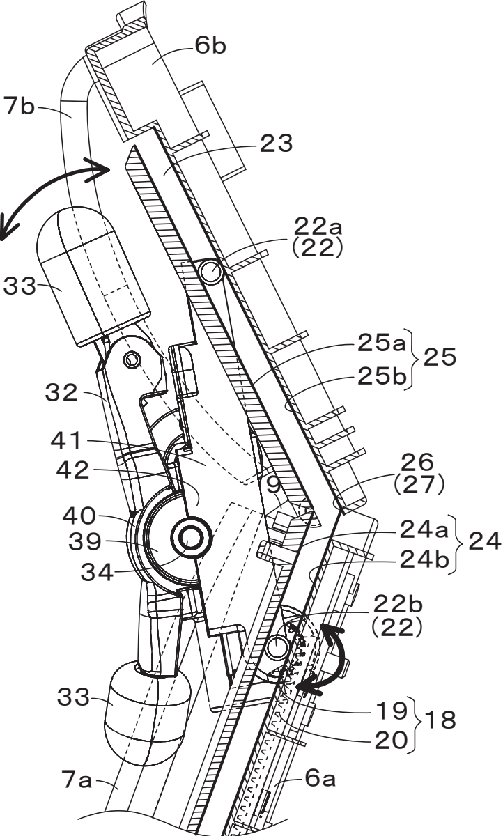
B-B cross section
