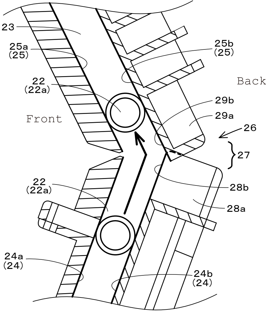
Enlargement of D part
