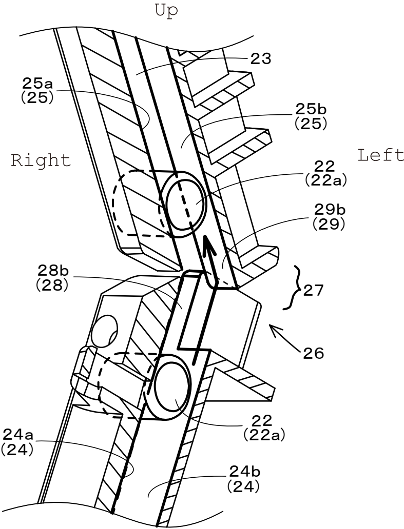
Enlargement of D part
