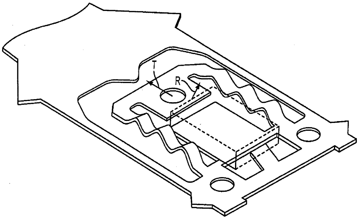
FIG. 2 PRIOR ART
