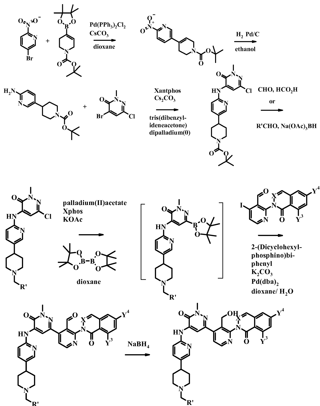
Scheme 6.
