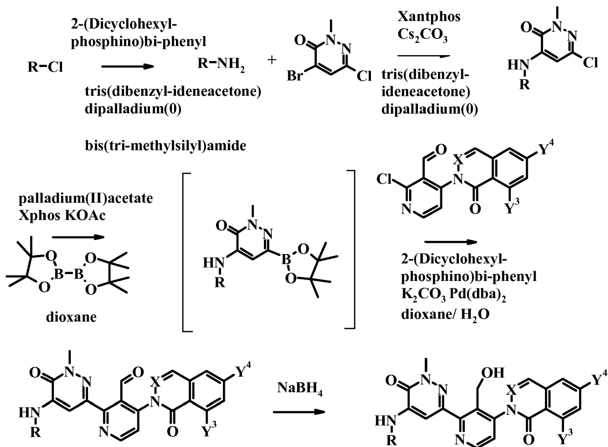
Scheme 11.
