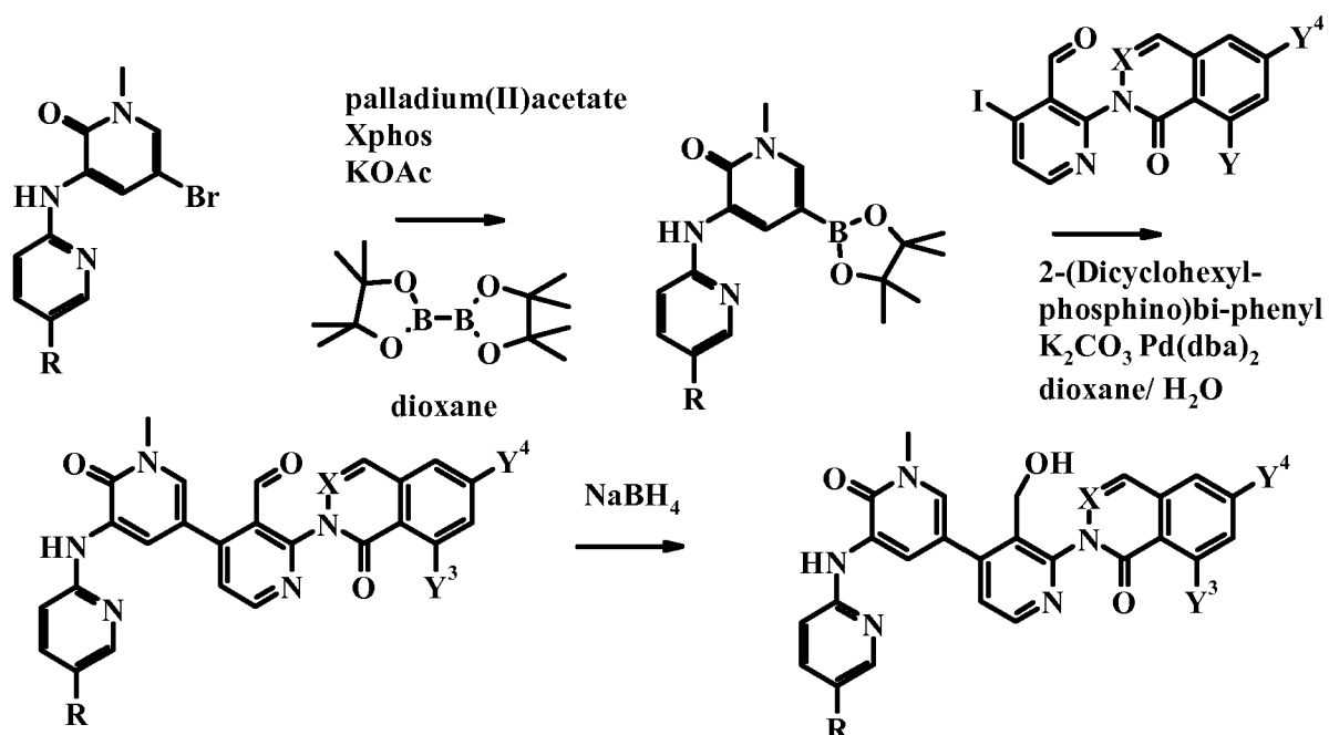
Scheme 10.
