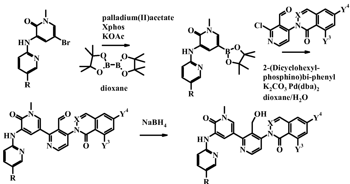
Scheme 10.
