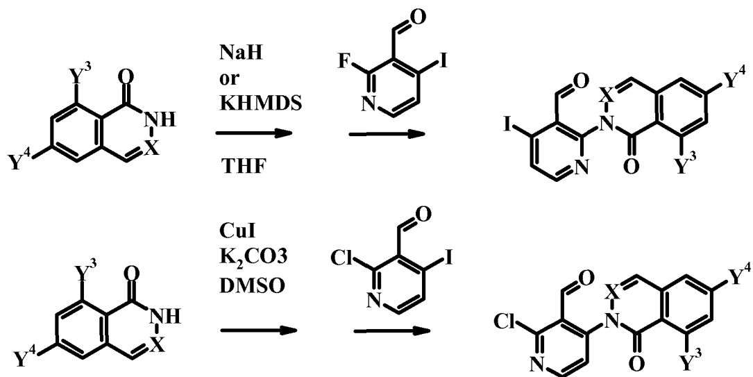
Scheme 4.
