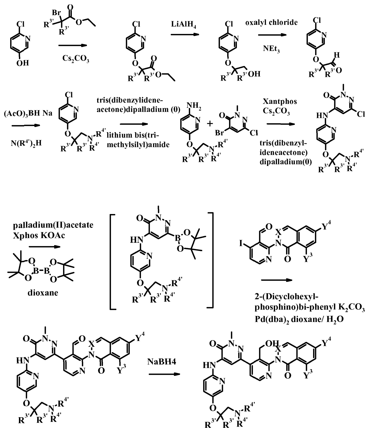
Scheme 7.
